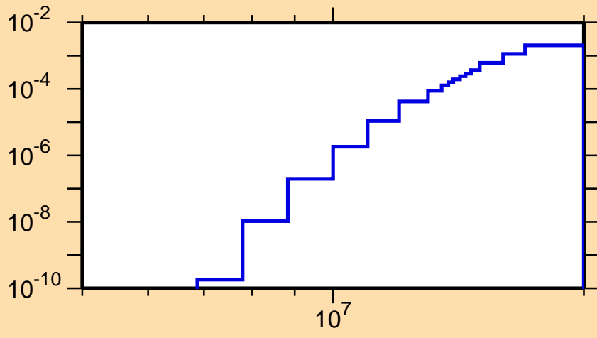
\sigma vs. E for ^{247}\text{Pu}(n,p)
