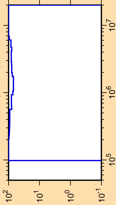
\Delta\sigma/\sigma vs. E for ^{247}\text{Pu}(n,\text{inel.})
