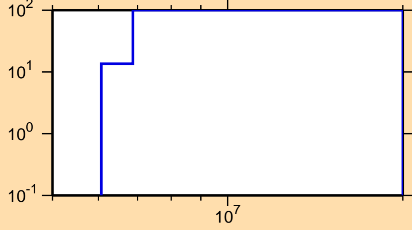
\Delta\sigma/\sigma vs. E for ^{247}\text{Pu}(n,p)
