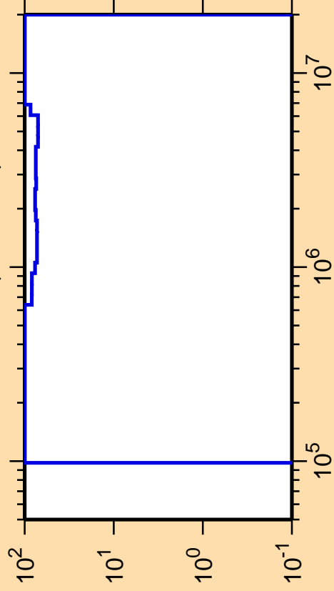
\Delta\sigma/\sigma vs. E for ^{247}\text{Pu}(n,\text{ncont.})
