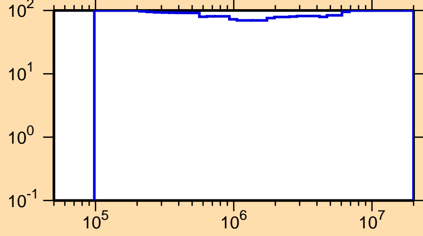
\Delta\sigma/\sigma vs. E for ^{247}\text{Pu}(n,\text{inel.})
