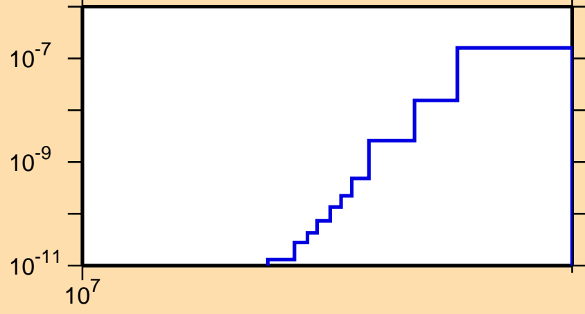
\sigma vs. E for ^{247}\text{Pu}(n,2n\alpha)
