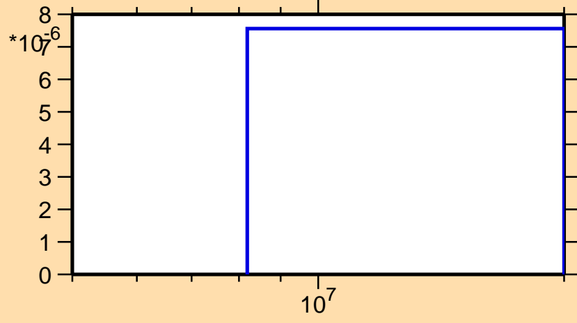
\sigma vs. E for ^{247}\text{Pu}(n,d)
