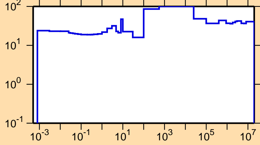
\Delta\sigma/\sigma vs. E for ^{247}\text{Pu}(n,\text{tot.})
