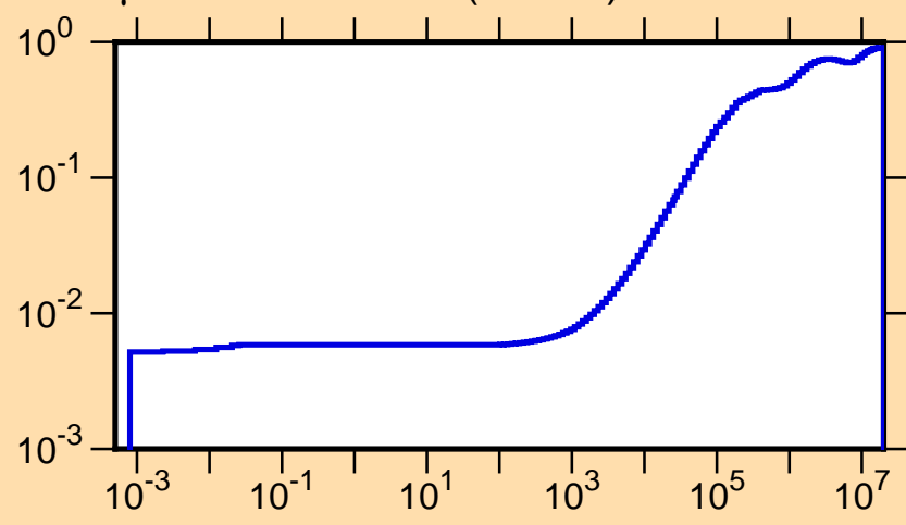
\mu vs. E for ^{131}\text{Sm}(\text{mt251})
