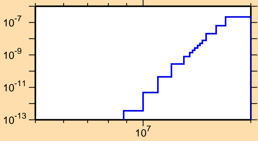
\sigma vs. E for ^{131}\text{Sm}(\text{mt117})
