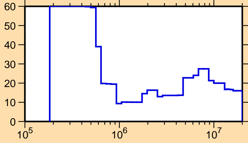
\Delta\sigma/\sigma vs. E for ^{131}\text{Sm}(n,\text{tot.})
