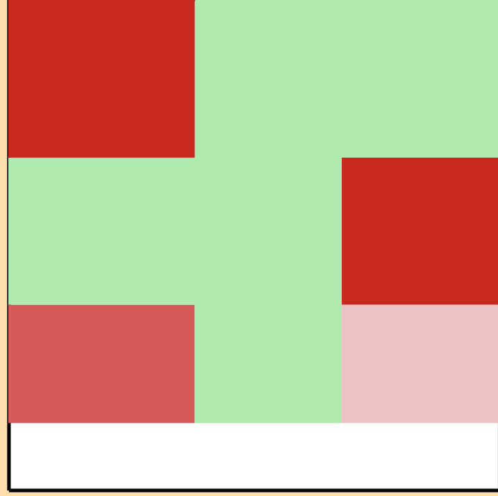
\Delta\sigma/\sigma vs. E for ^{131}\text{Sm}(n,\text{nonel.})
