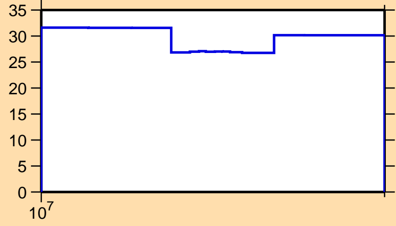
\Delta\sigma/\sigma vs. E for ^{131}\text{Sm}(n,\text{el.})
