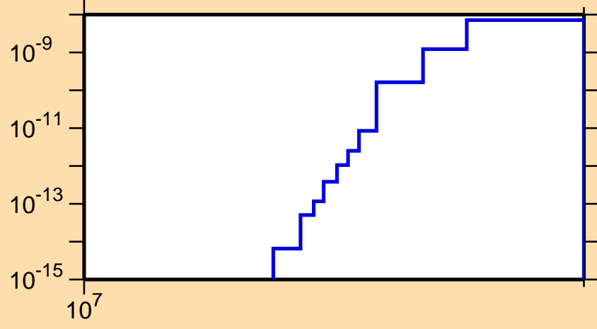
\sigma vs. E for ^{131}\text{Sm}(n,2n\alpha)
