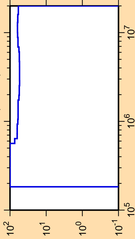
\Delta\sigma/\sigma vs. E for ^{131}\text{Sm}(n,\text{inel.})
