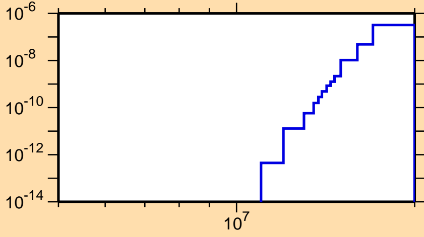
\sigma vs. E for ^{131}\text{Sm} (mt 34)
