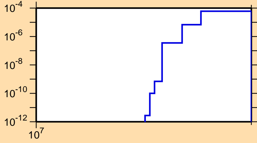
\sigma vs. E for ^{131}\text{Sm}(n,2np)
