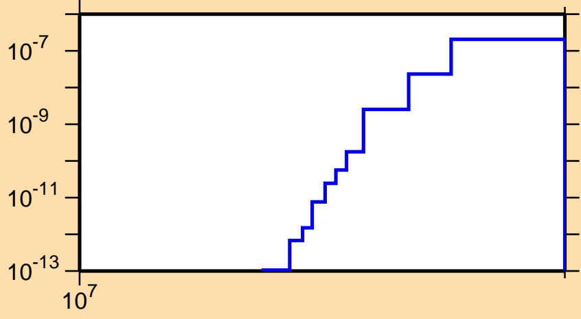
\sigma vs. E for ^{131}\text{Sm}(n,\text{nd})
