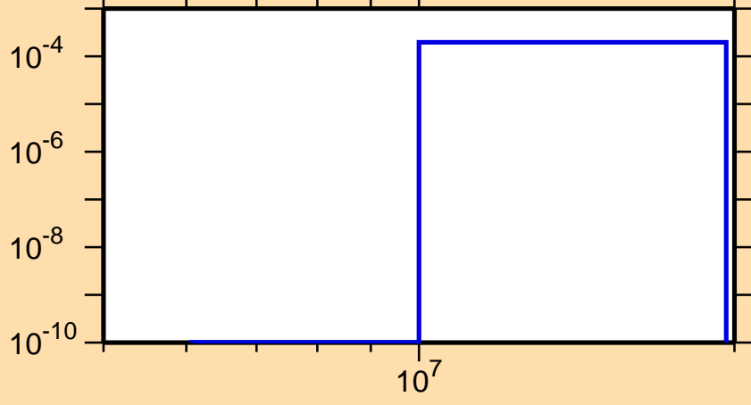
\sigma vs. E for ^{131}\text{Sm}(n,t)
