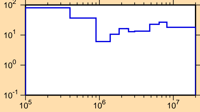
\Delta\sigma/\sigma vs. E for ^{131}\text{Sm}(n,\text{tot.})
