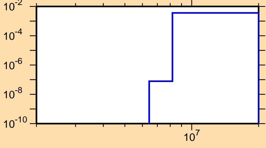
\sigma vs. E for ^{131}\text{Sm}(n,pd)
