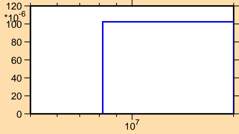
\sigma vs. E for ^{131}\text{Sm}(n,\text{pt})
