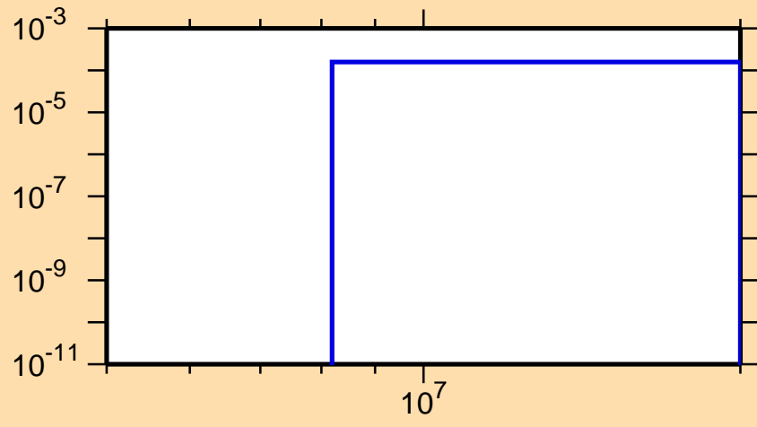
\sigma vs. E for ^{131}\text{Sm}(n,t)
