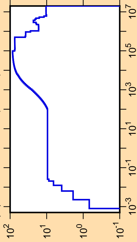
\Delta\mu/\mu vs. E for ^{132}\text{Sm}(\text{mt251})
