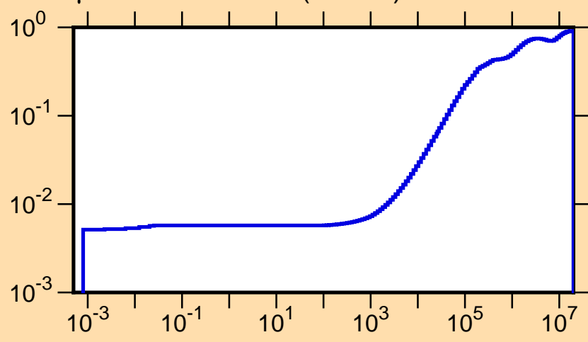
\mu vs. E for ^{132}\text{Sm}(\text{mt251})
