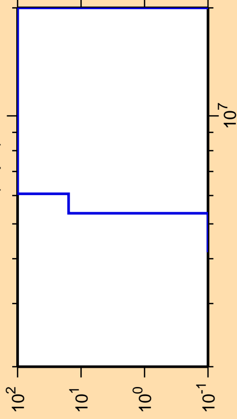
\Delta\sigma/\sigma vs. E for ^{132}\text{Sm}(n,\text{pd})
