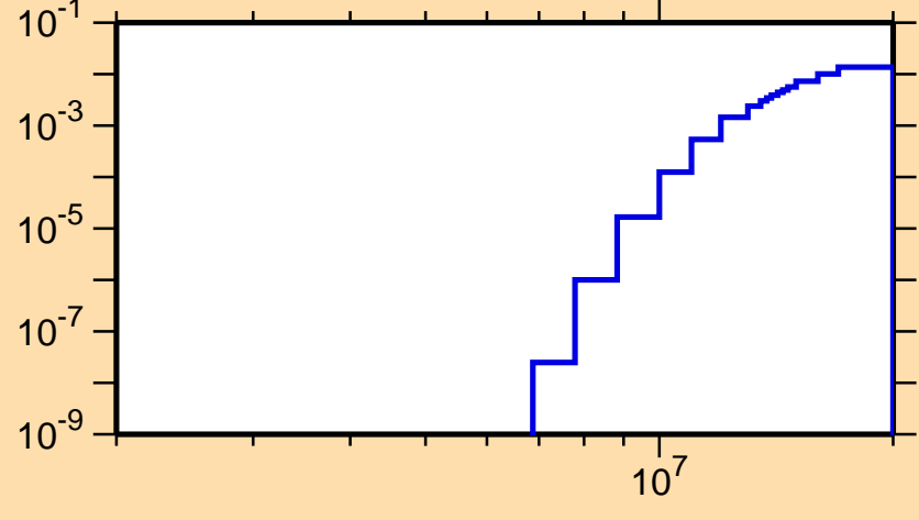
\sigma vs. E for ^{132}\text{Sm}(n,\text{pd})
