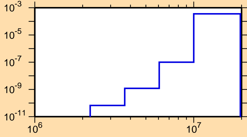
\sigma vs. E for ^{132}\text{Sm}(n,\text{He3})
