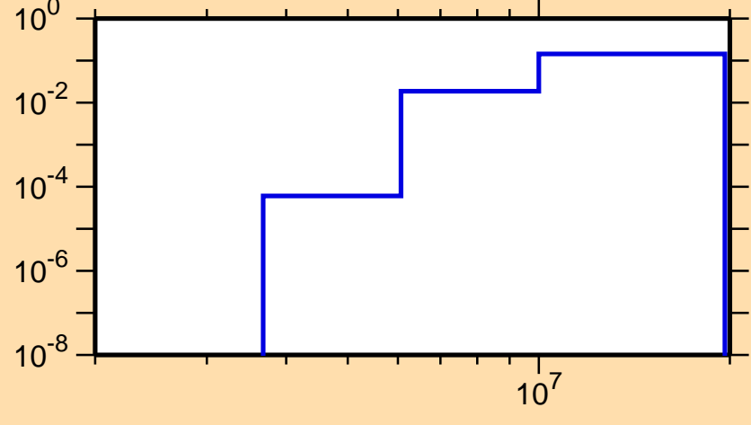
\sigma vs. E for ^{132}\text{Sm}(n,np)
