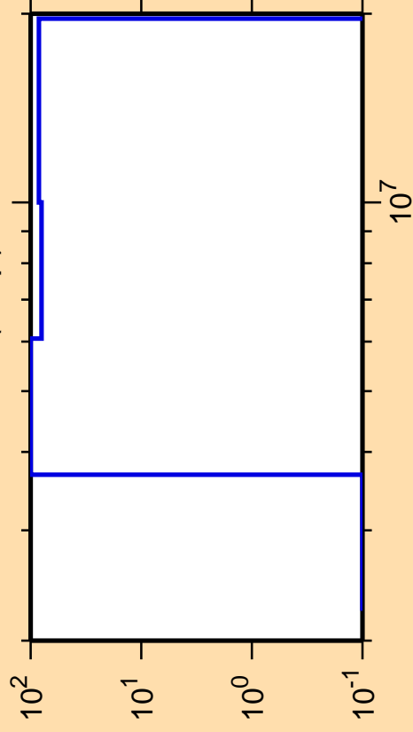
\Delta\sigma/\sigma vs. E for ^{132}\text{Sm}(n,np)
