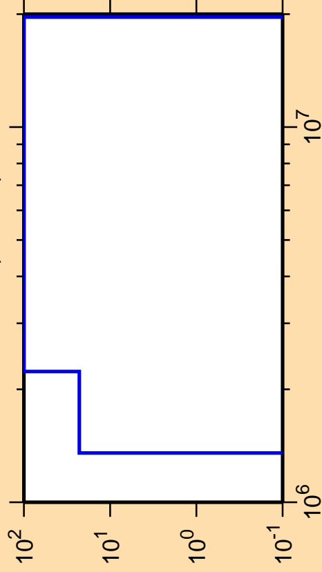
\Delta\sigma/\sigma vs. E for ^{132}\text{Sm}(n,\text{He3})
