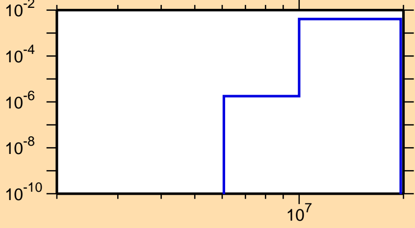
\sigma vs. E for ^{132}\text{Sm}(n,pd)
