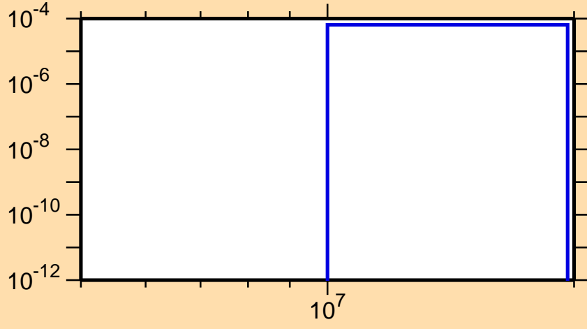
\sigma vs. E for ^{132}\text{Sm}(n,t)
