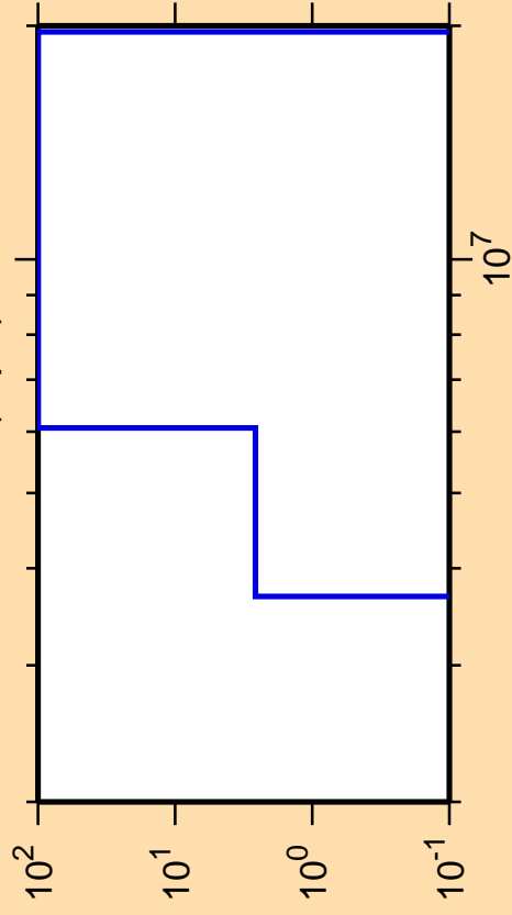
\Delta\sigma/\sigma vs. E for ^{132}\text{Sm}(n,pd)
