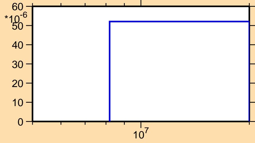
\sigma vs. E for ^{132}\text{Sm}(n,t)
