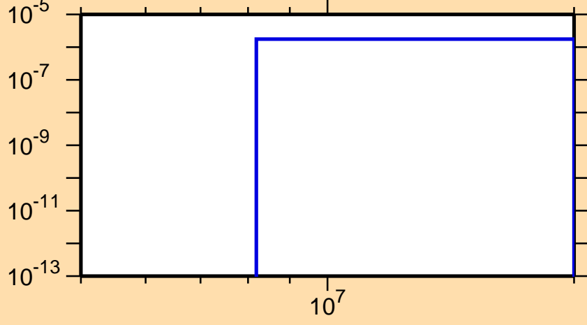
\sigma vs. E for ^{132}\text{Sm} (mt 45)
