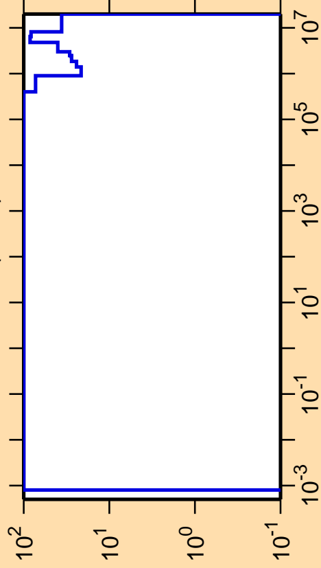
\Delta\sigma/\sigma vs. E for ^{132}\text{Sm}(n,\text{el.})
