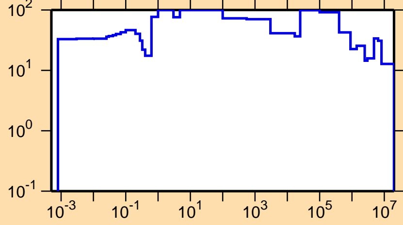
\Delta\sigma/\sigma vs. E for ^{132}\text{Sm}(n,\text{tot.})
