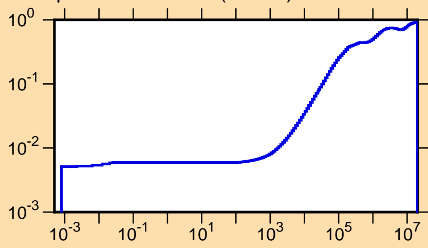
\mu vs. E for ^{133}\text{Sm}(\text{mt251})
