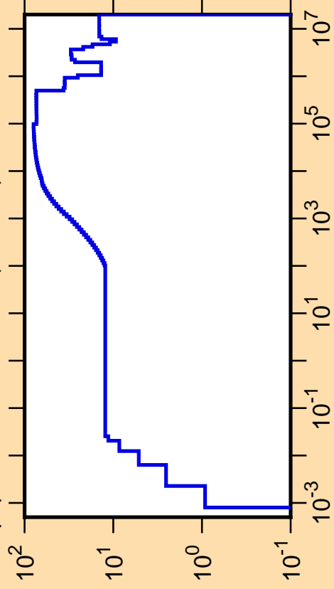
\Delta\mu/\mu vs. E for ^{133}\text{Sm}(\text{mt251})
