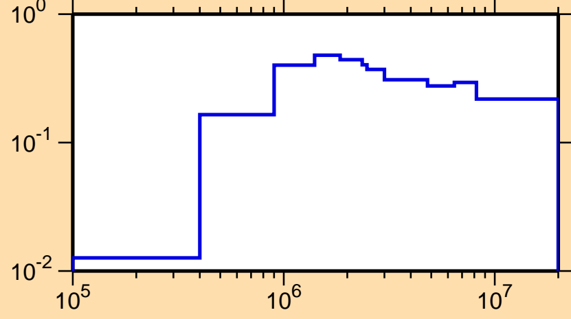
\sigma vs. E for ^{133}\text{Sm}(n,\text{inel.})
