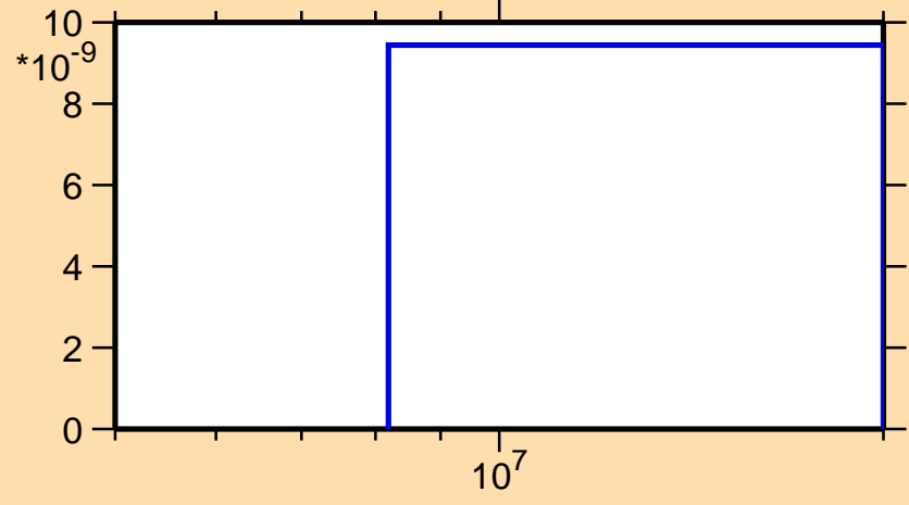
\sigma vs. E for ^{133}\text{Sm} (mt 34)
