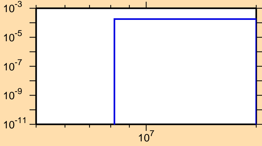
\sigma vs. E for ^{133}\text{Sm}(n,t)
