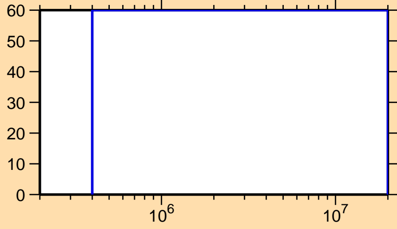
\Delta\sigma/\sigma vs. E for ^{133}\text{Sm}(n,ncont.)
