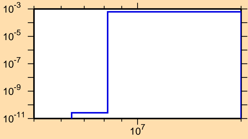
\sigma vs. E for ^{133}\text{Sm}(n,\text{pd})
