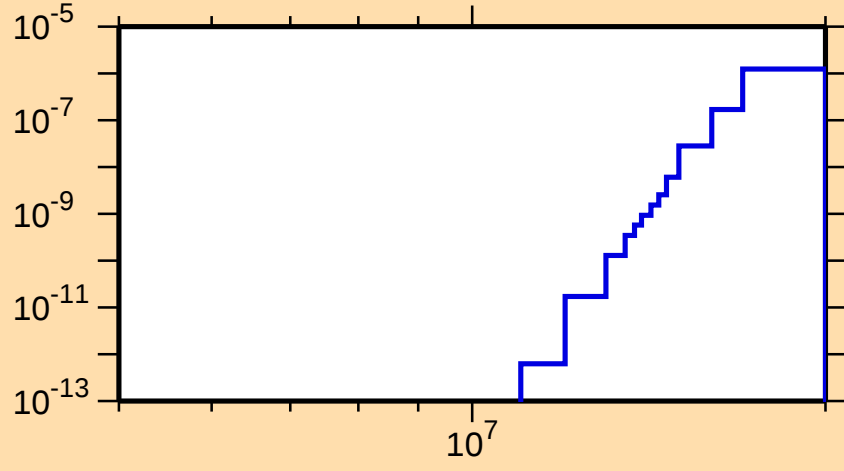
\sigma vs. E for ^{133}\text{Sm}(\text{mt } 34)
