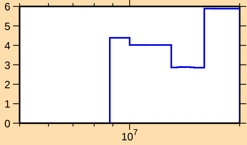
\Delta\sigma/\sigma vs. E for ^{133}\text{Sm}(n,\text{tot.})
