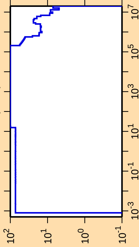
\Delta\sigma/\sigma vs. E for ^{133}\text{Sm}(n,\text{el.})
