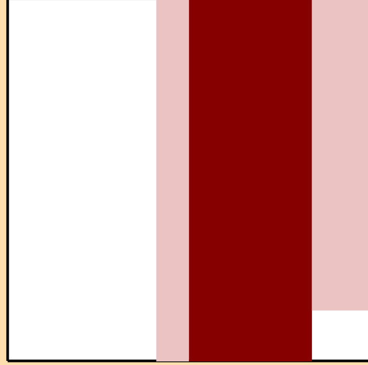
\Delta\sigma/\sigma vs. E for ^{133}\text{Sm}(n,2n)
