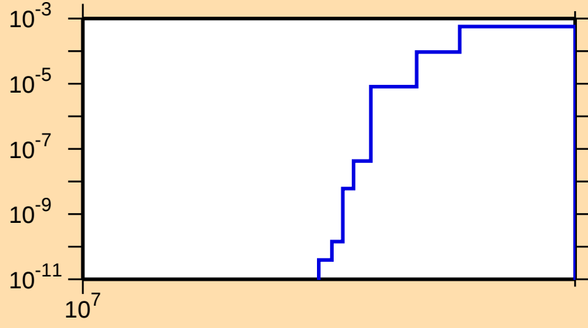
\sigma vs. E for ^{133}\text{Sm}(n,2np)
