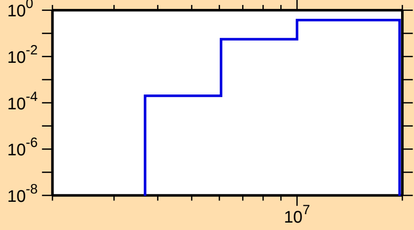
\sigma vs. E for ^{133}\text{Sm}(n,np)
