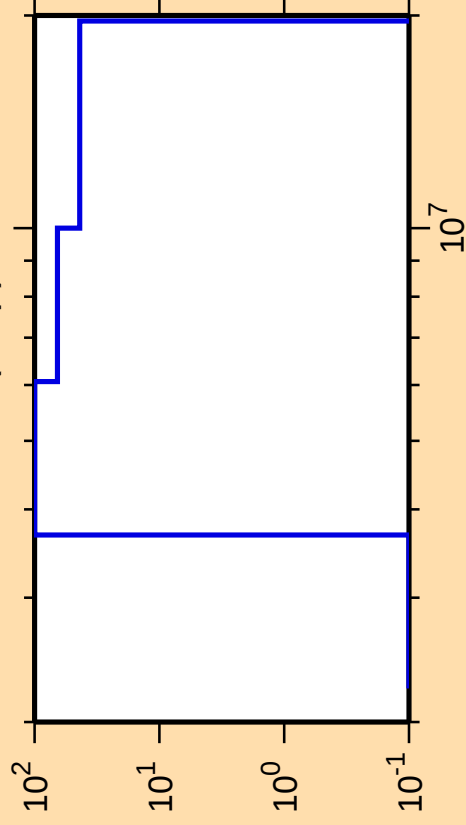
\Delta\sigma/\sigma vs. E for ^{133}\text{Sm}(n,np)
