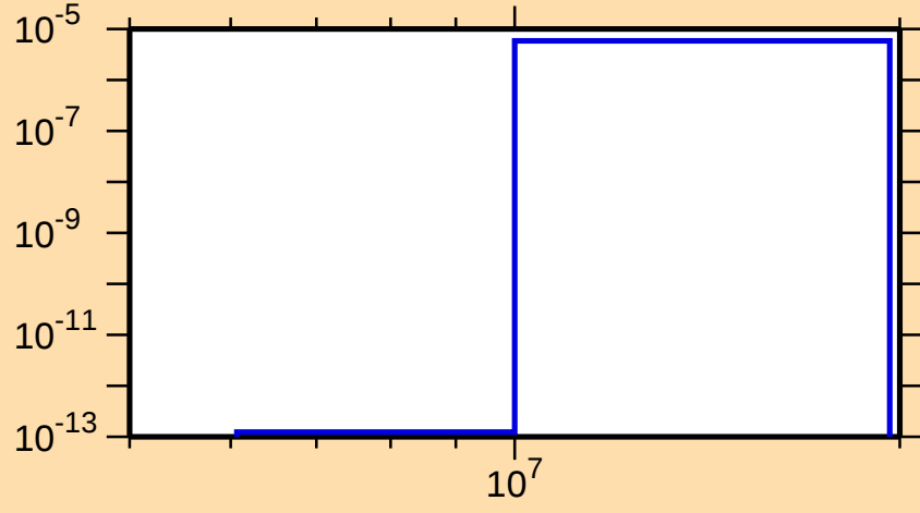
\sigma vs. E for ^{133}\text{Sm}(\text{mt } 45)
