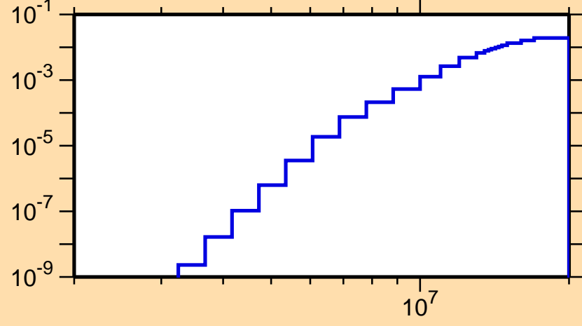
\sigma vs. E for ^{134}\text{Sm}(n,n\alpha)
