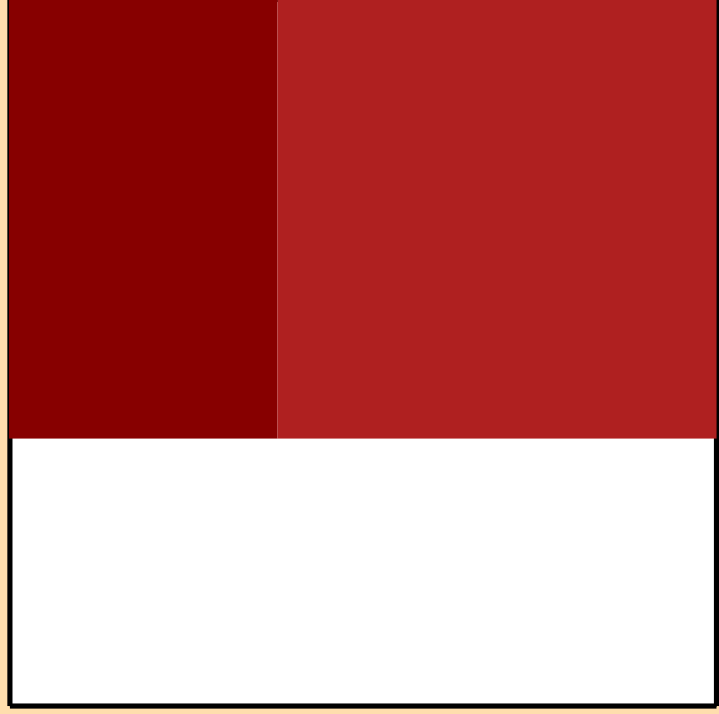
\Delta\sigma/\sigma vs. E for ^{134}\text{Sm}(n,\text{tot.})
