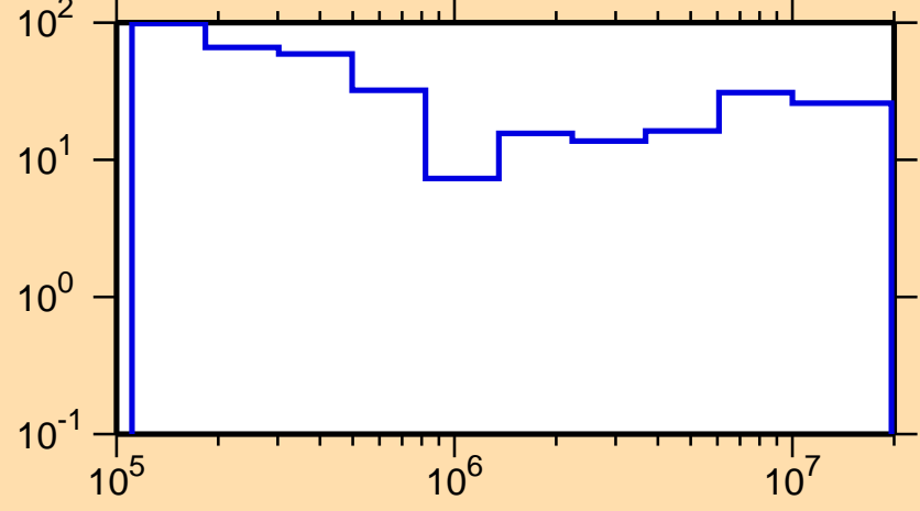
\Delta\sigma/\sigma vs. E for ^{134}\text{Sm}(n,\text{tot.})
