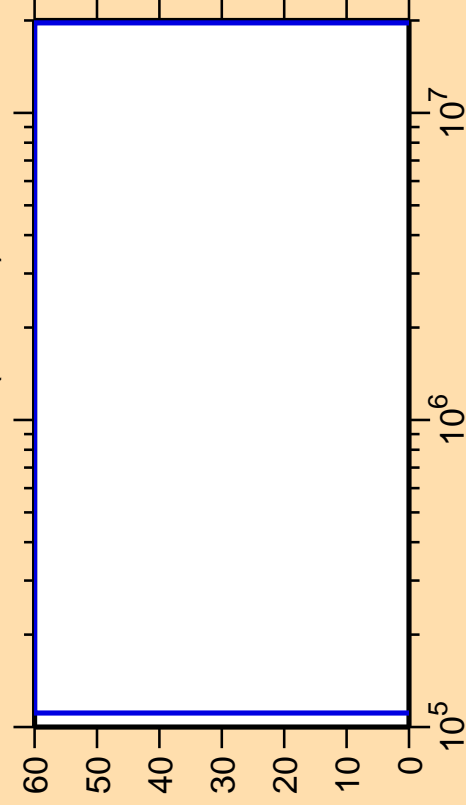
\Delta\sigma/\sigma vs. E for ^{134}\text{Sm}(n,\text{inel.})
