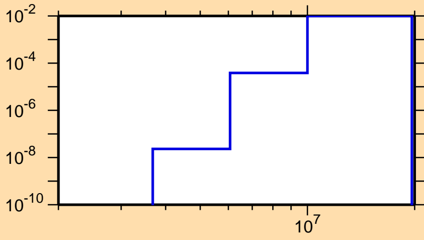
\sigma vs. E for ^{134}\text{Sm}(n,d)
