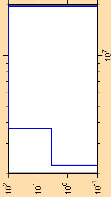
\Delta\sigma/\sigma vs. E for ^{134}\text{Sm}(n,d)
