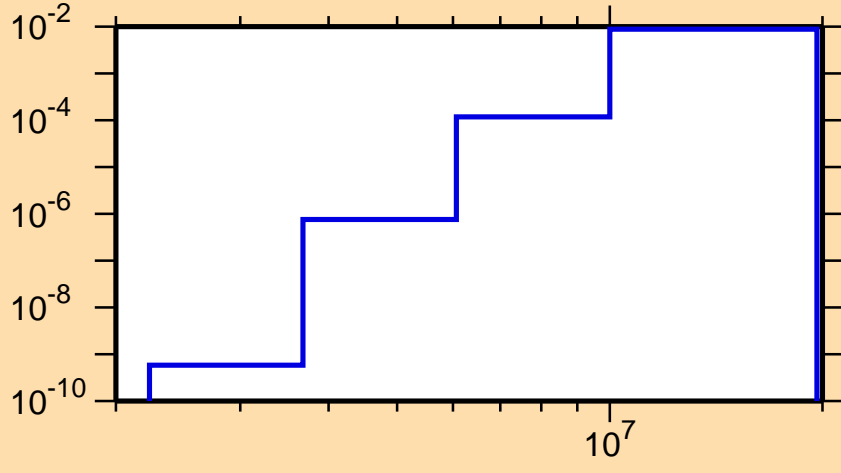
\sigma vs. E for ^{134}\text{Sm}(n,n\alpha)
