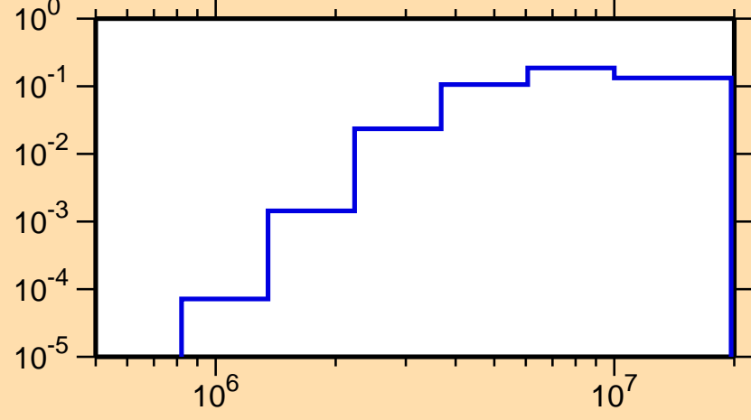
\sigma vs. E for ^{134}\text{Sm}(n,n\text{cont.})
