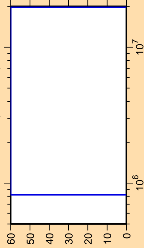
\Delta\sigma/\sigma vs. E for ^{134}\text{Sm}(n,n\text{cont.})
