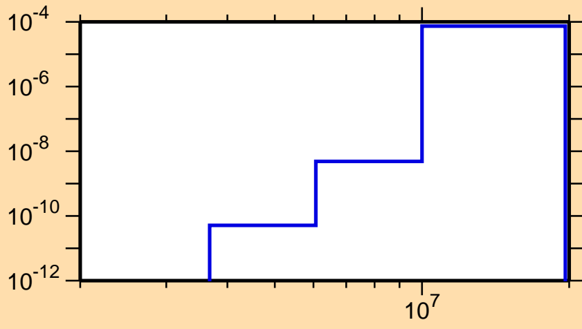
\sigma vs. E for ^{134}\text{Sm}(n,\text{He3})
