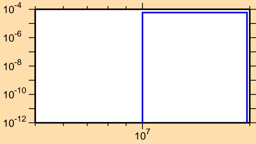
\sigma vs. E for ^{134}\text{Sm}(n,t)
