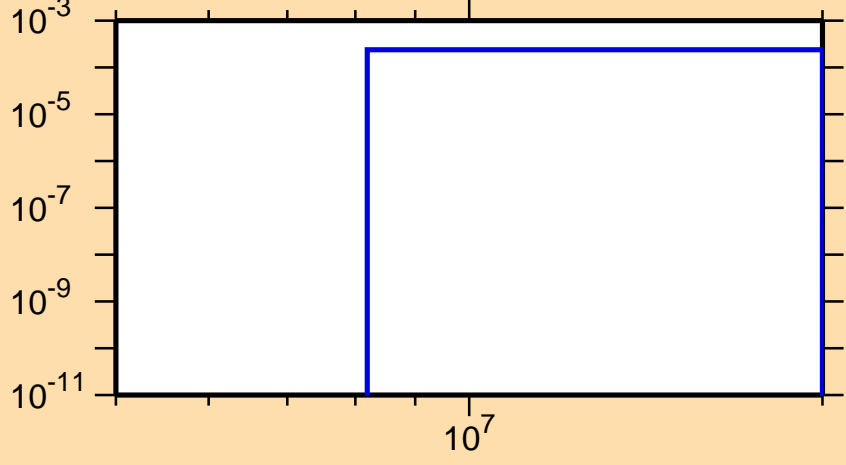
\sigma vs. E for ^{134}\text{Sm}(n,\text{pd})
