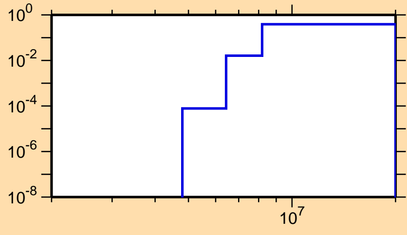
\sigma vs. E for ^{134}\text{Sm}(n,np)
