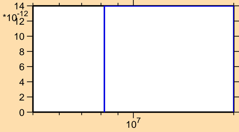
\sigma vs. E for ^{134}\text{Sm}(\text{mt } 34)
