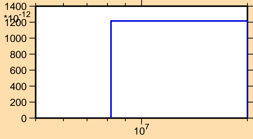
\sigma vs. E for ^{134}\text{Sm}(\text{mt117})
