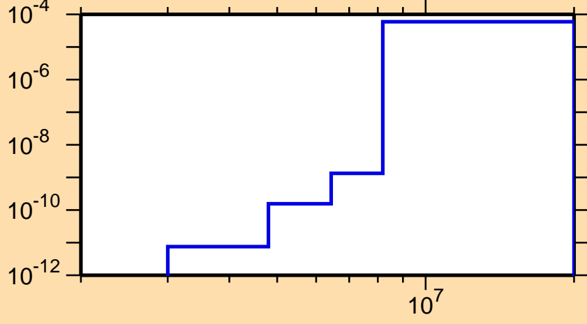
\sigma vs. E for ^{134}\text{Sm}(n,\text{He3})
