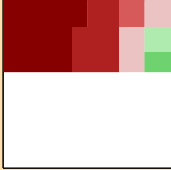
\Delta\sigma/\sigma vs. E for ^{135}\text{Sm}(n,\text{tot.})
