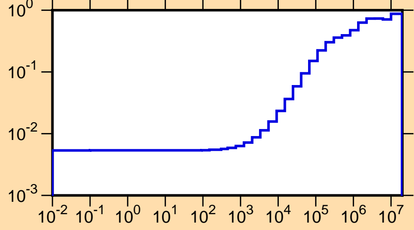
\mu vs. E for ^{135}\text{Sm}(\text{mt251})
