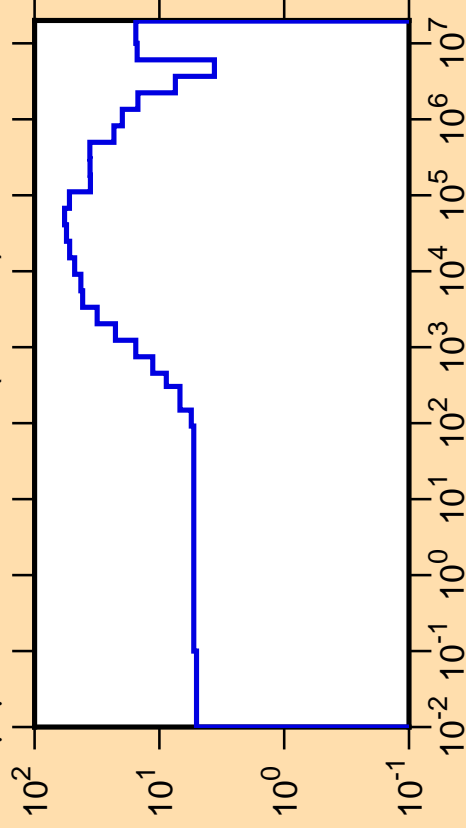
\Delta\mu/\mu vs. E for ^{135}\text{Sm}(\text{mt251})
