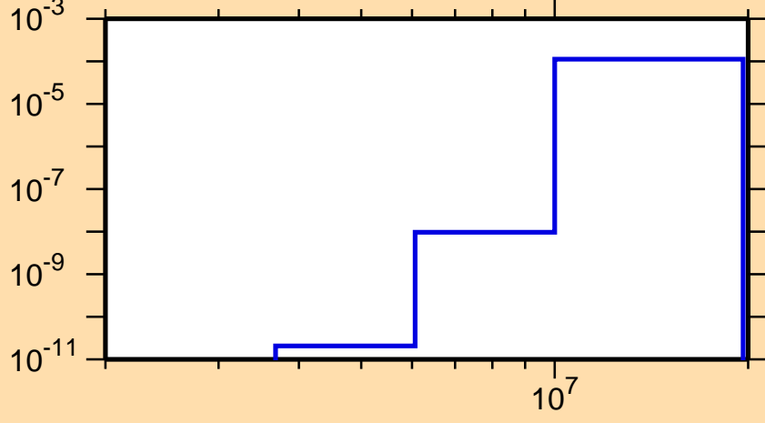
\sigma vs. E for ^{135}\text{Sm}(n,\text{He3})
