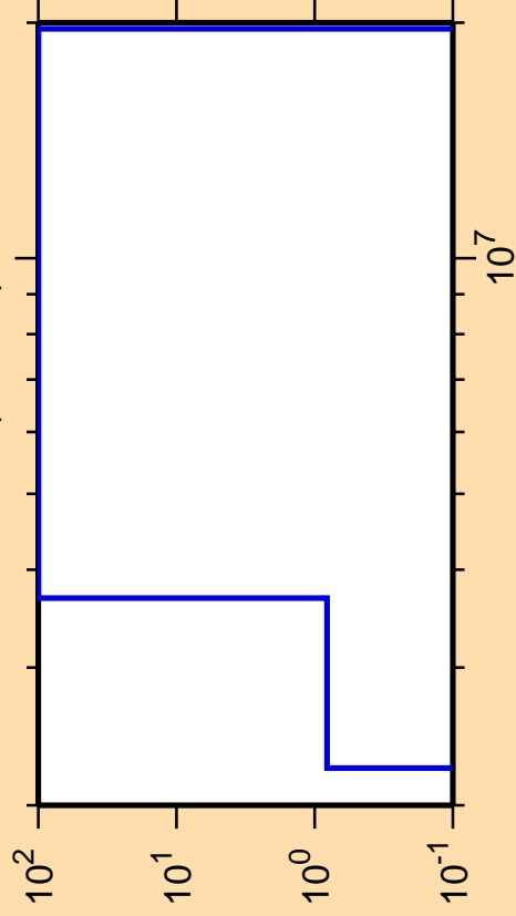
\Delta\sigma/\sigma vs. E for ^{135}\text{Sm}(n,\text{He3})
