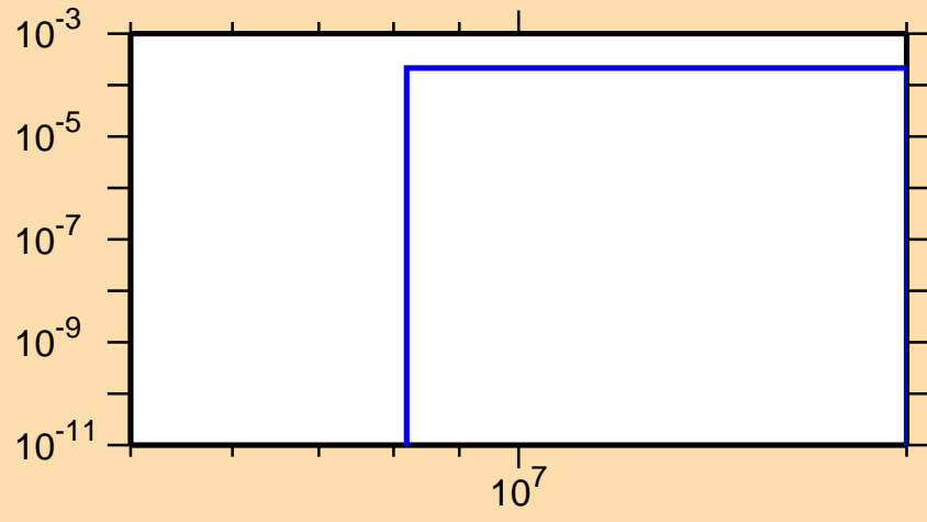
\sigma vs. E for ^{135}\text{Sm}(n,t)
