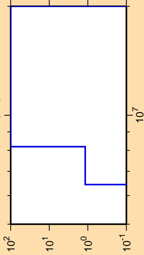
\Delta\sigma/\sigma vs. E for ^{135}\text{Sm}(n,t)
