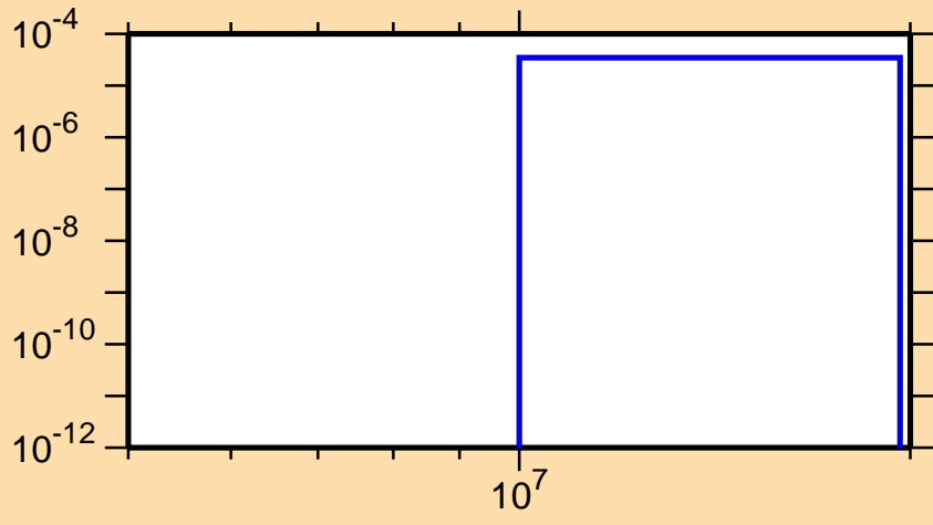
\sigma vs. E for ^{136}\text{Sm}(n,t)
