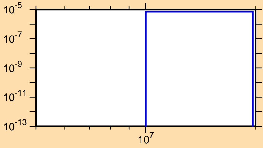
\sigma vs. E for ^{136}\text{Sm}(\text{mt } 45)
