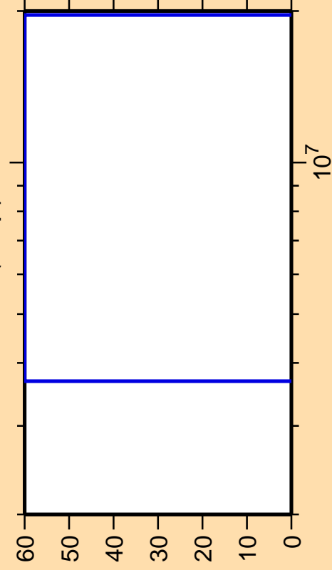
\Delta\sigma/\sigma vs. E for ^{136}\text{Sm}(n,np)
