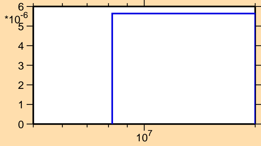
\sigma vs. E for ^{136}\text{Sm}(\text{mt } 45)
