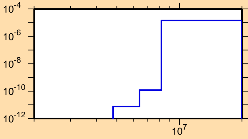
\sigma vs. E for ^{136}\text{Sm}(n,\text{He3})
