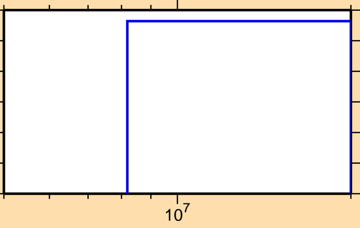
\sigma vs. E for ^{136}\text{Sm}(\text{mt } 45)
