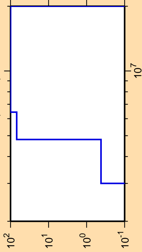
\Delta\sigma/\sigma vs. E for ^{136}\text{Sm}(n,\text{He3})
