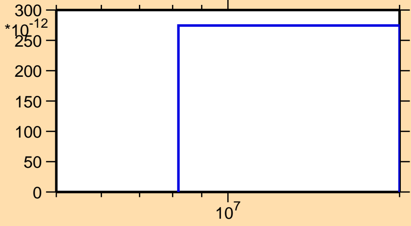
\sigma vs. E for ^{136}\text{Sm}(n,nd)
