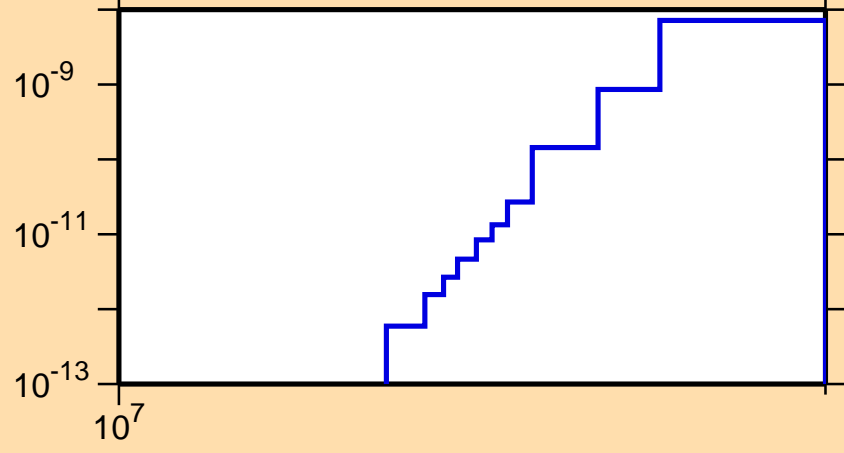
\sigma vs. E for ^{137}\text{Sm}(\text{mt117})
