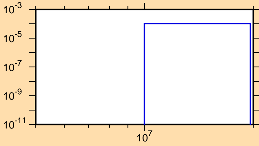
\sigma vs. E for ^{137}\text{Sm}(n,t)
