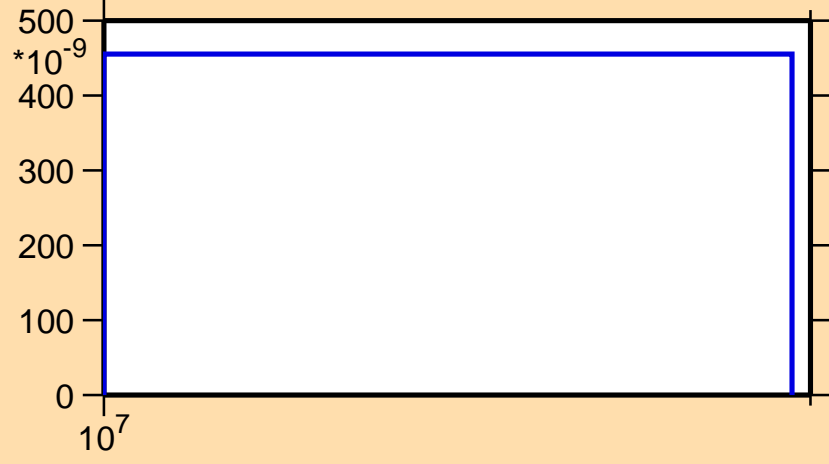
\sigma vs. E for ^{137}\text{Sm}(n,pt)
