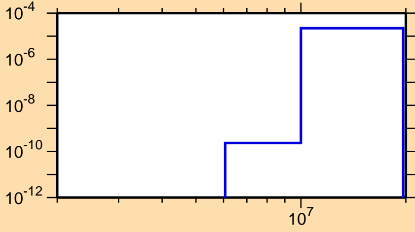
\sigma vs. E for ^{137}\text{Sm}(n,\text{He3})
