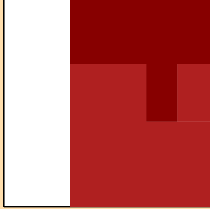
\Delta\sigma/\sigma vs. E for ^{139}\text{Sm}(n,2n)
