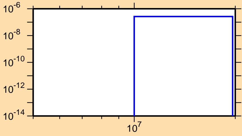
\sigma vs. E for ^{139}\text{Sm}(n,\text{pd})
