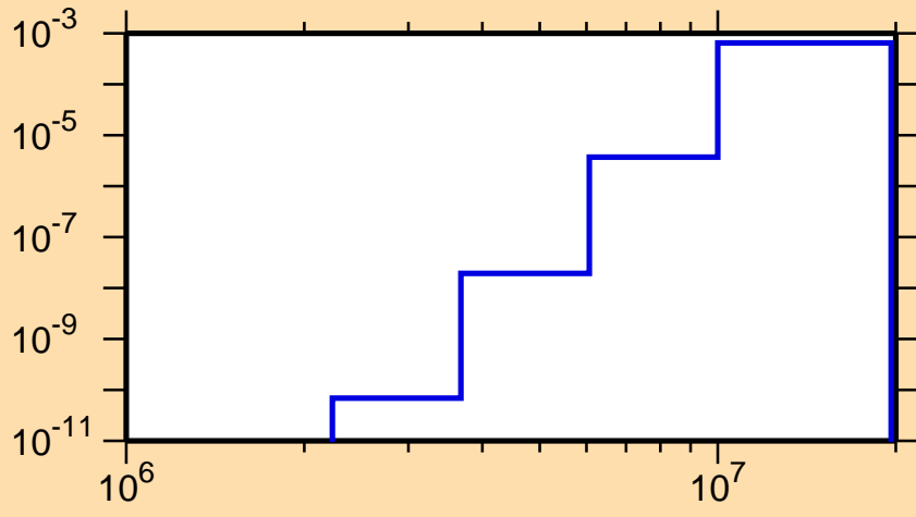
\sigma vs. E for ^{139}\text{Sm}(n,p\alpha)
