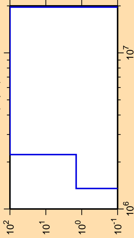
\Delta\sigma/\sigma vs. E for ^{139}\text{Sm}(n,p\alpha)
