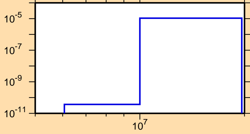
\sigma vs. E for ^{139}\text{Sm}(n,\text{He3})
