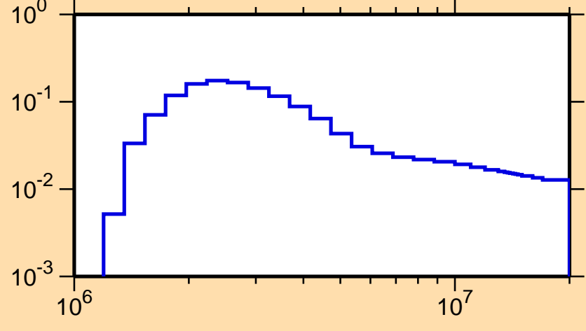
\sigma vs. E for ^{140}\text{Sm}(n,n_3)
