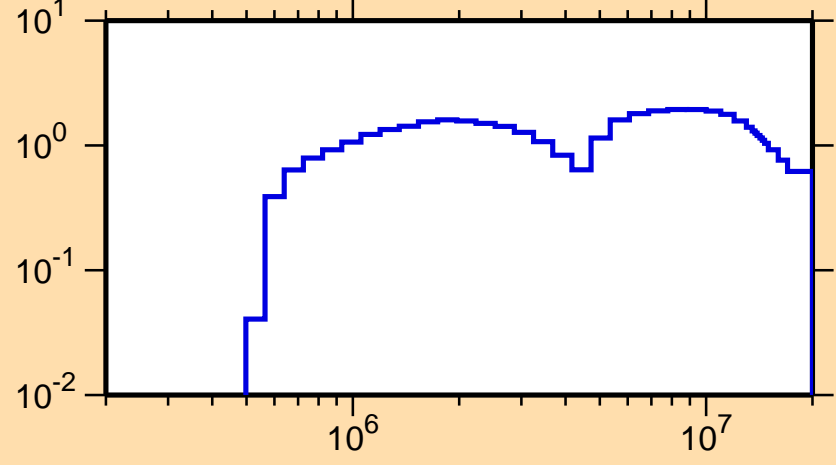
\sigma vs. E for ^{140}\text{Sm}(n,\text{inel.})
