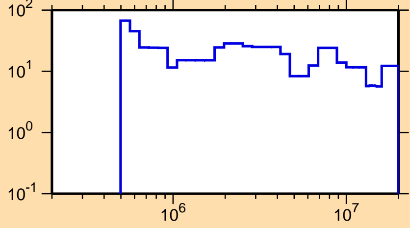
\Delta\sigma/\sigma vs. E for ^{140}\text{Sm}(n,\text{el.})
