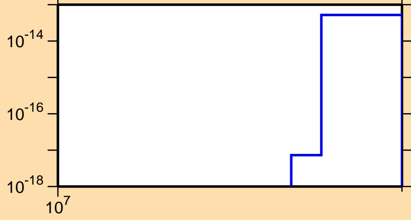
\sigma vs. E for ^{140}\text{Sm}(n,nt)
