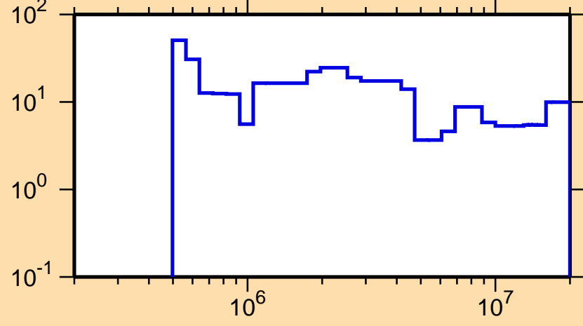
\Delta\sigma/\sigma vs. E for ^{140}\text{Sm}(n,\text{tot.})
