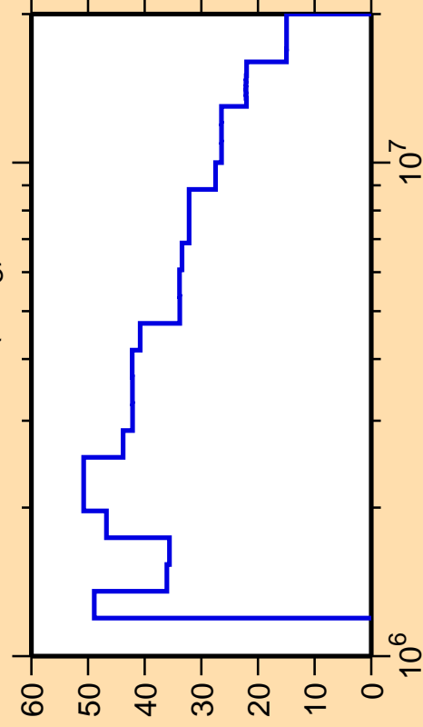
\Delta\sigma/\sigma vs. E for ^{140}\text{Sm}(n,n_3)
