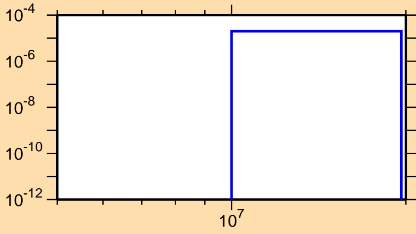
\sigma vs. E for ^{140}\text{Sm}(n,t)
