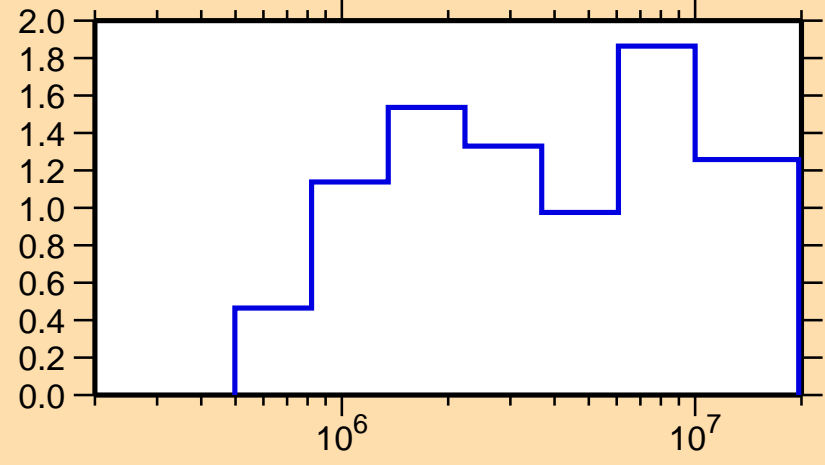
\sigma vs. E for ^{140}\text{Sm}(n,\text{inel.})
