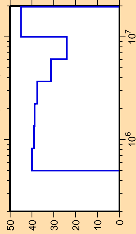
\Delta\sigma/\sigma vs. E for ^{140}\text{Sm}(n,\text{inel.})
