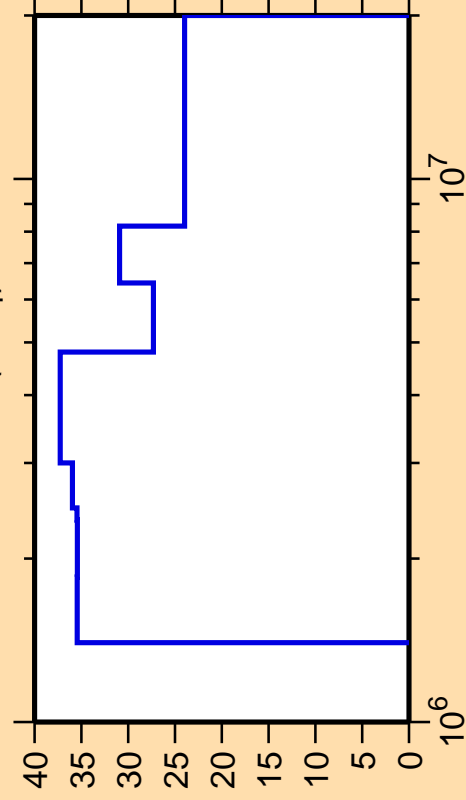
\Delta\sigma/\sigma vs. E for ^{140}\text{Sm}(n,n_4)
