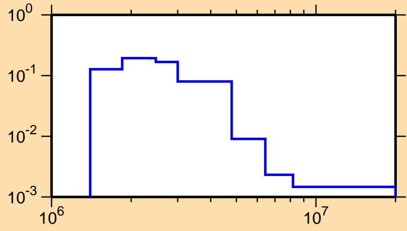
\sigma vs. E for ^{140}\text{Sm}(n,n_4)
