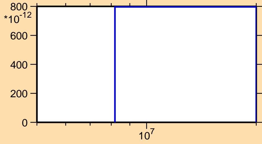
\sigma vs. E for ^{140}\text{Sm}(\text{mt } 45)
