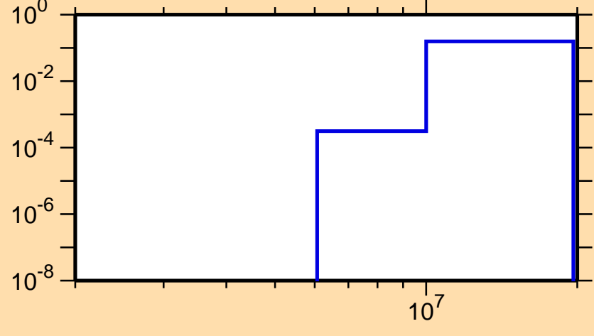
\sigma vs. E for ^{141}\text{Sm}(n,np)
