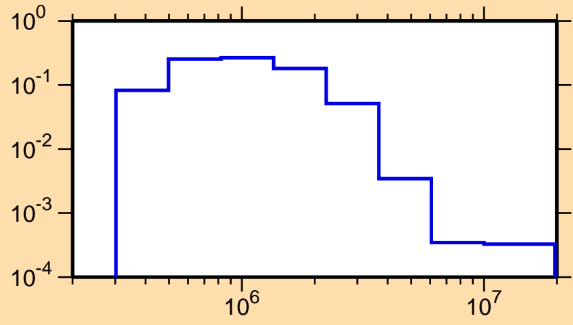
\sigma vs. E for ^{141}\text{Sm}(n,n_3)
