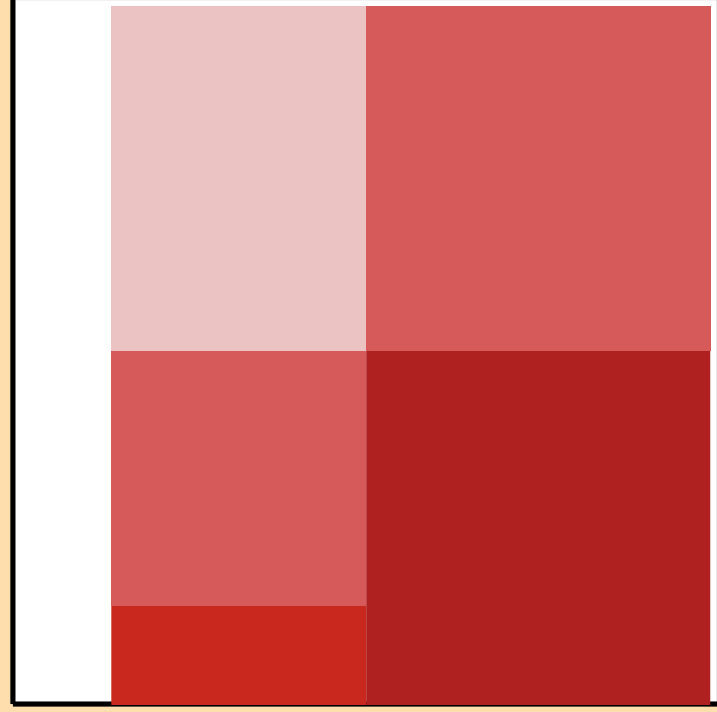
\Delta\sigma/\sigma vs. E for ^{141}\text{Sm}(n,2n)
