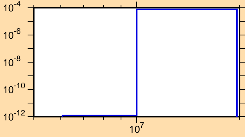
\sigma vs. E for ^{141}\text{Sm}(n,t)
