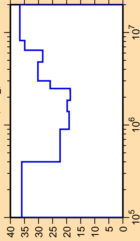
\Delta\sigma/\sigma vs. E for ^{141}\text{Sm}(n,n_2)
