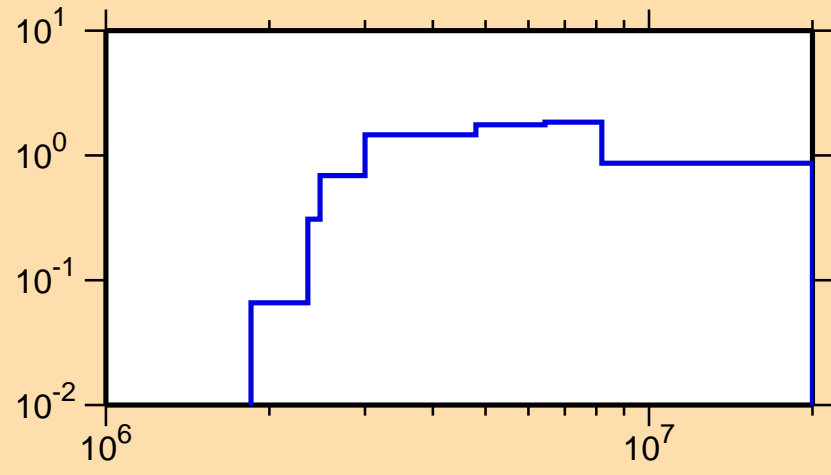
\sigma vs. E for ^{141}\text{Sm}(n,n\text{cont.})
