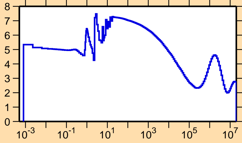
\sigma vs. E for ^{141}\text{Sm}(n,\text{el.})
