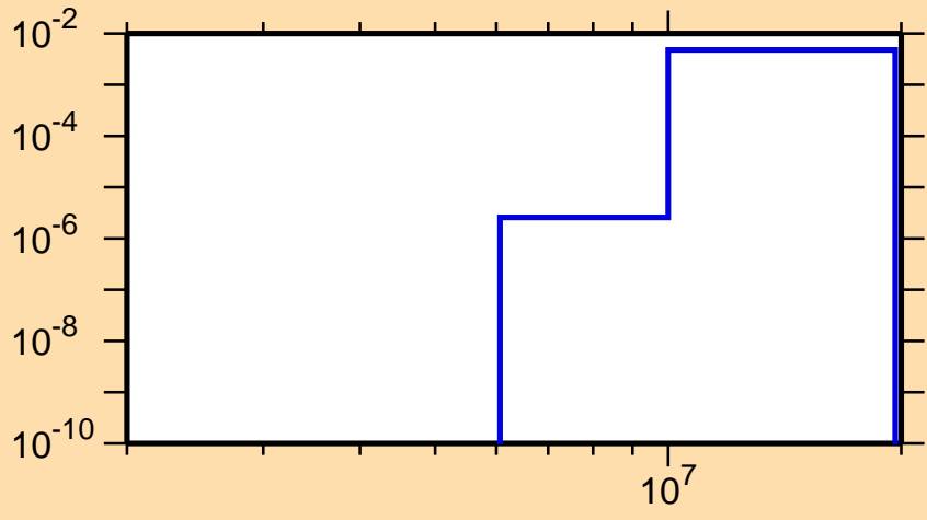
\sigma vs. E for ^{141}\text{Sm}(n,d)
