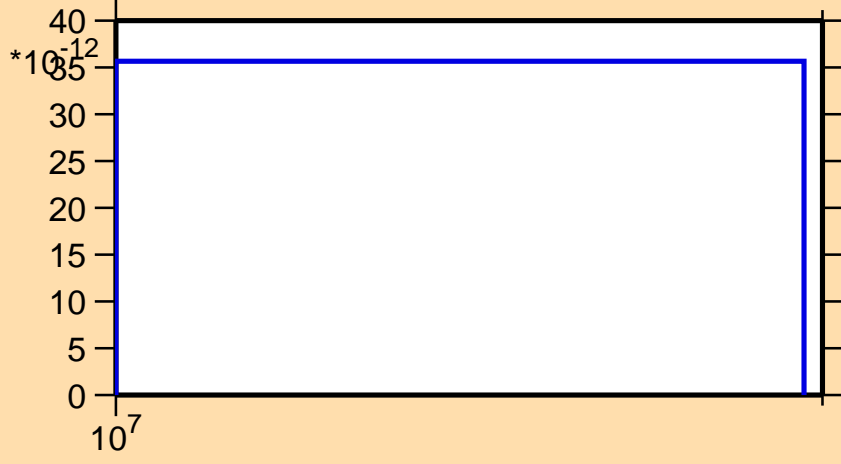
\sigma vs. E for ^{141}\text{Sm} (mt 45)
