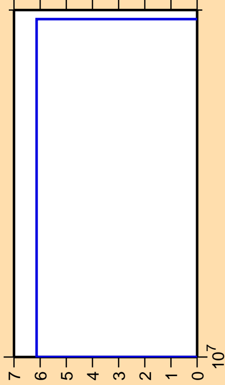
\Delta\sigma/\sigma vs. E for ^{141}\text{Sm}(\text{mt117})
