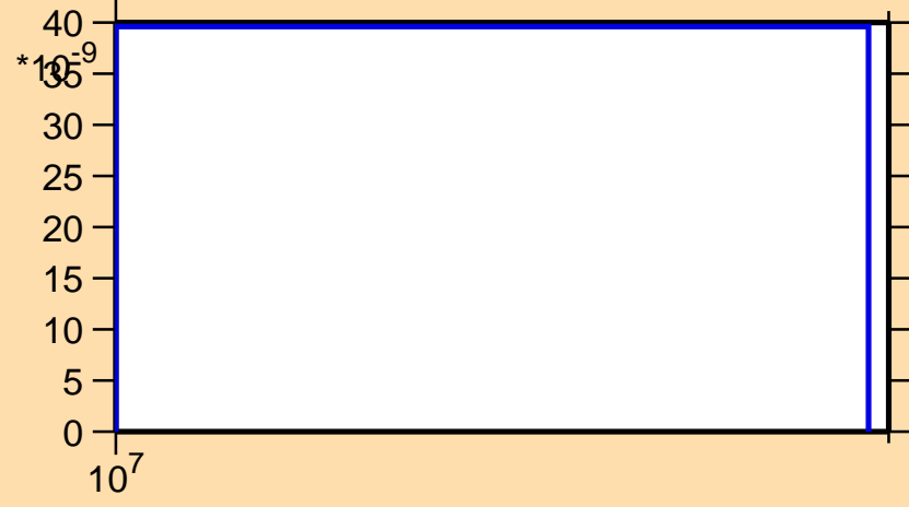
\sigma vs. E for ^{141}\text{Sm}(n,\text{nd})
