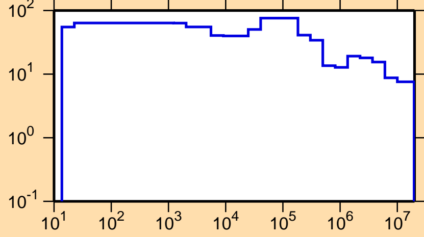
\Delta\sigma/\sigma vs. E for ^{141}\text{Sm}(n,\text{tot.})
