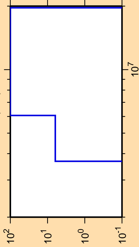
\Delta\sigma/\sigma vs. E for ^{141}\text{Sm}(n,d)
