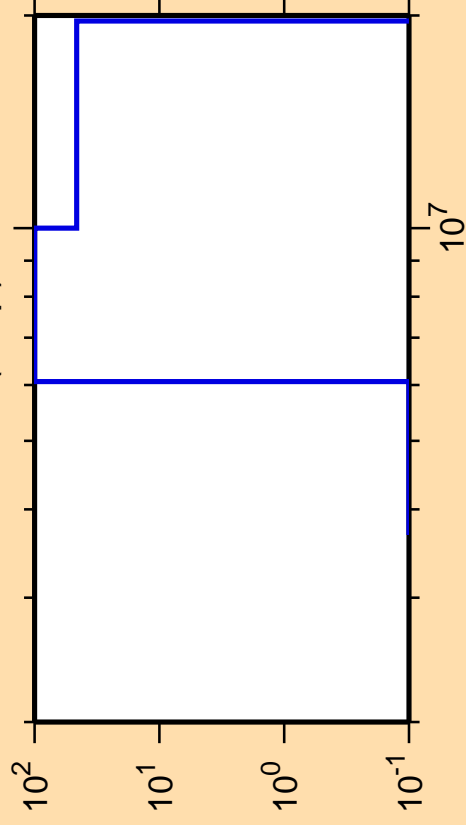
\Delta\sigma/\sigma vs. E for ^{141}\text{Sm}(n,np)
