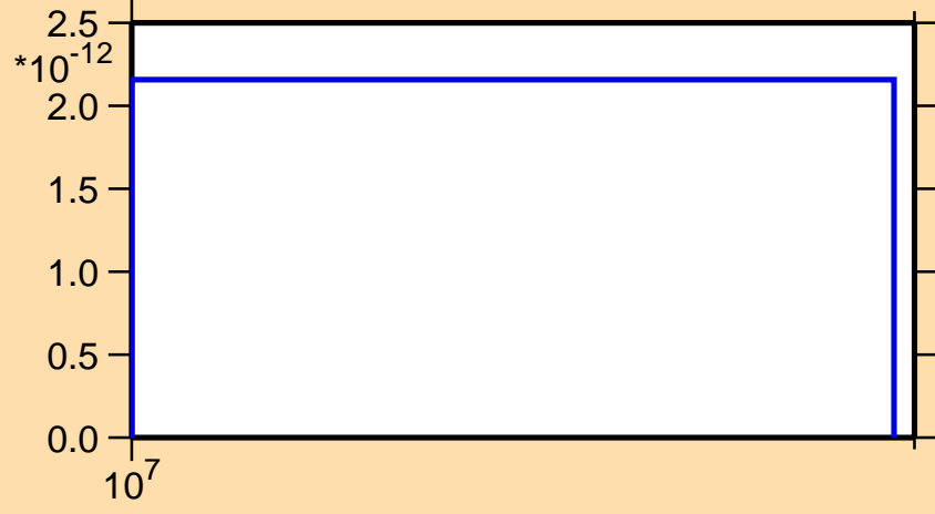
\sigma vs. E for ^{141}\text{Sm} (mt 34)
