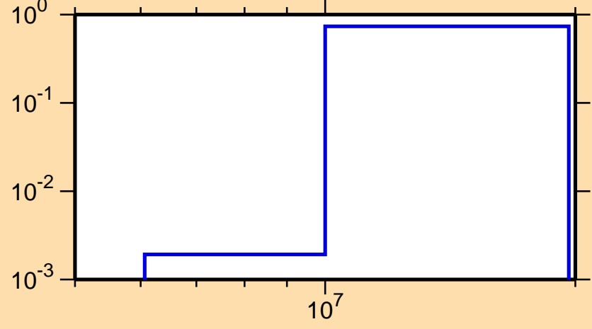
\sigma vs. E for ^{141}\text{Sm}(n,2n)
