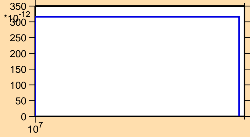
\sigma vs. E for ^{141}\text{Sm}(n,\text{pt})
