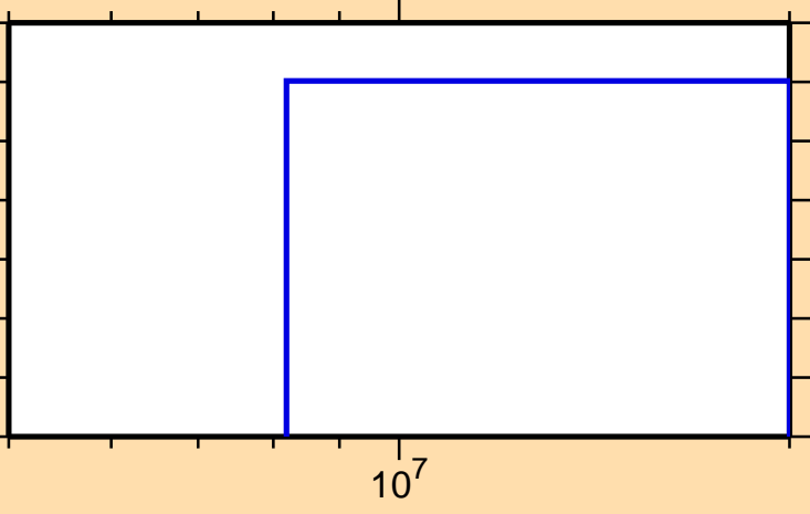
\sigma vs. E for ^{141}\text{Sm}(n,2np)
