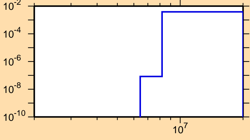
\sigma vs. E for ^{141}\text{Sm}(n,d)
