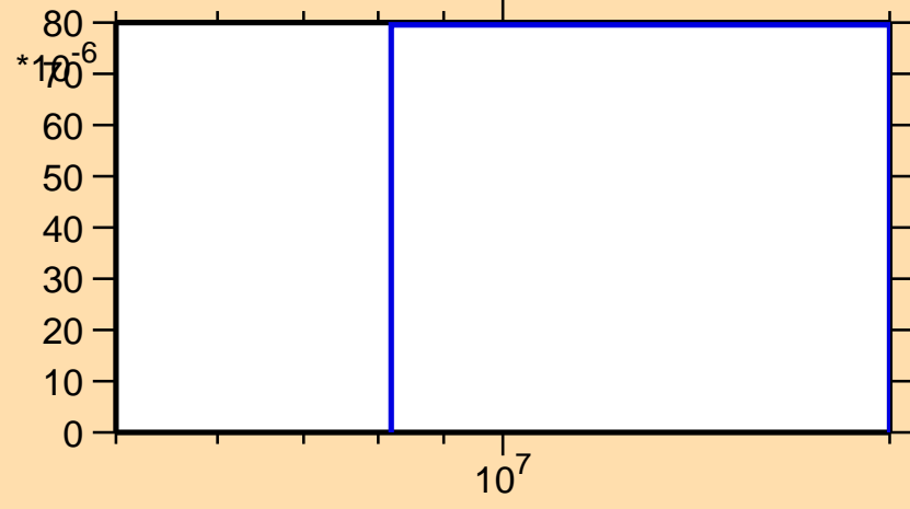
\sigma vs. E for ^{141}\text{Sm}(n,t)
