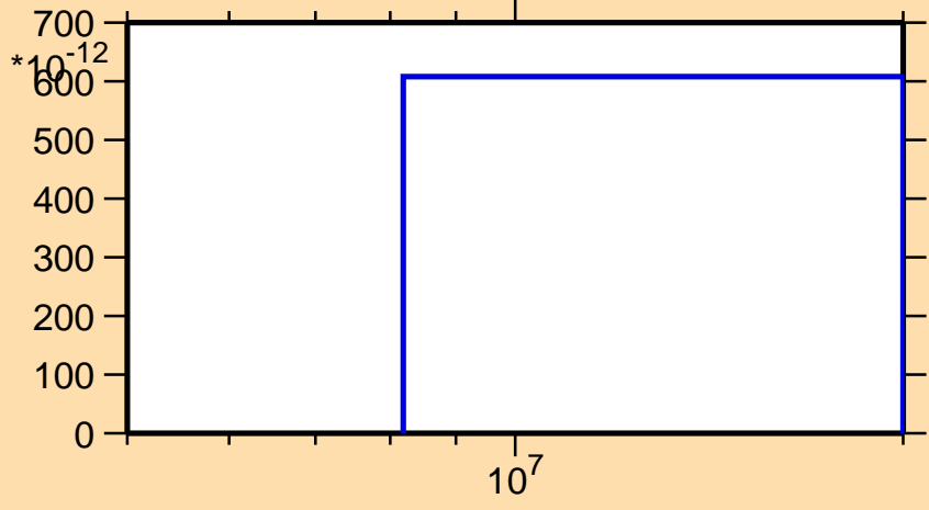
\sigma vs. E for ^{141}\text{Sm}(n,3n)
