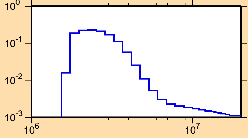
\sigma vs. E for ^{142}\text{Sm}(n,n_4)
