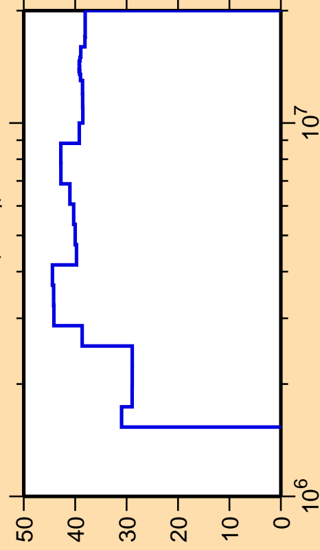
\Delta\sigma/\sigma vs. E for ^{142}\text{Sm}(n,n_4)
