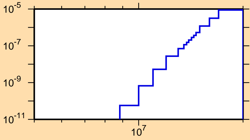
\sigma vs. E for ^{142}\text{Sm}(n,p\alpha)
