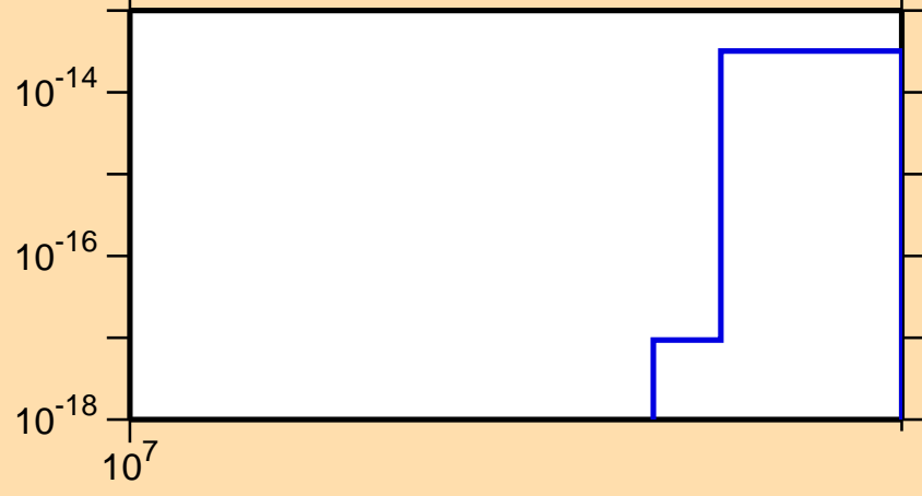
\sigma vs. E for ^{142}\text{Sm}(n,nt)
