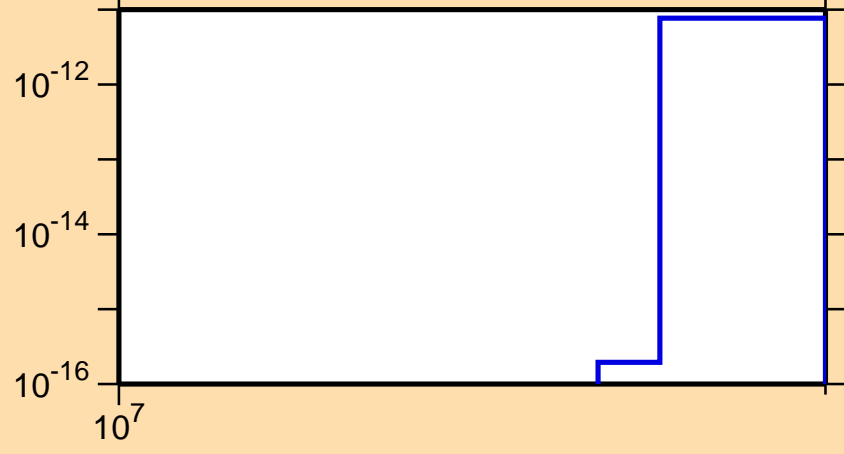
\sigma vs. E for ^{142}\text{Sm}(n,\text{pt})
