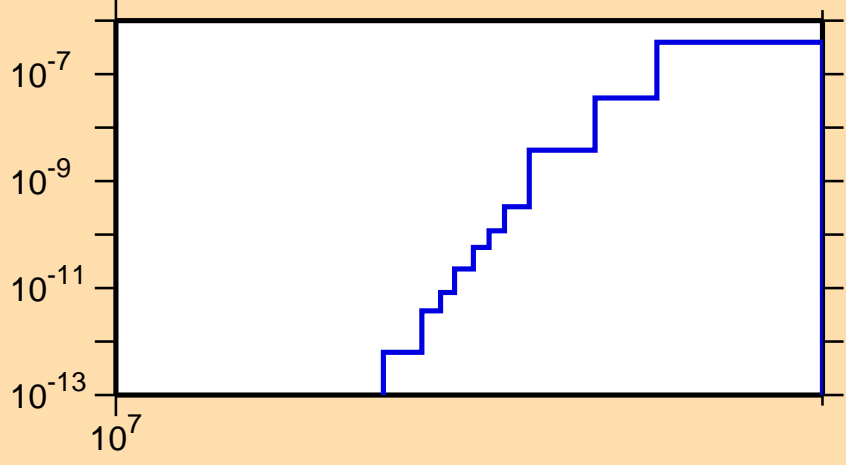
\sigma vs. E for ^{142}\text{Sm}(n,pd)
