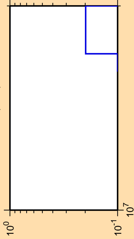
\Delta\sigma/\sigma vs. E for ^{142}\text{Sm}(n,nt)
