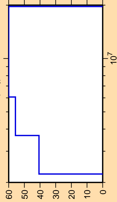
\Delta\sigma/\sigma vs. E for ^{142}\text{Sm}(n,\gamma)
