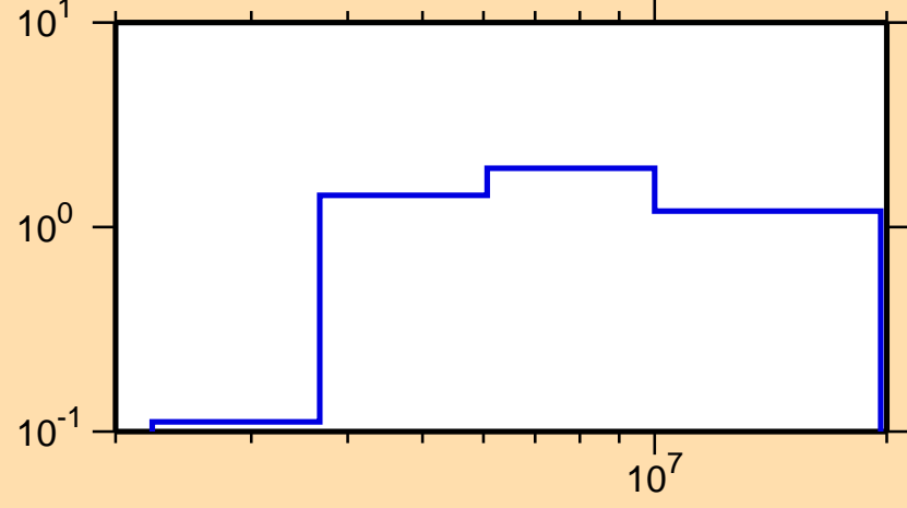
\sigma vs. E for ^{142}\text{Sm}(n,n\text{cont.})
