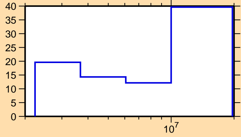
\Delta\sigma/\sigma vs. E for ^{142}\text{Sm}(n,ncont.)
