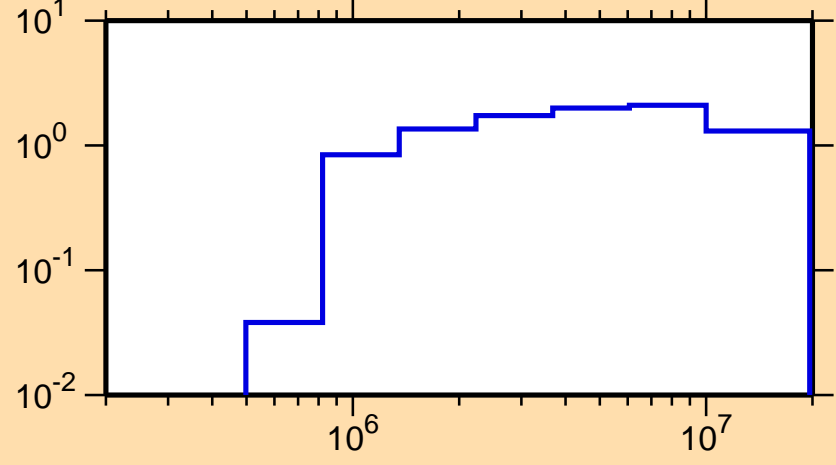
\sigma vs. E for ^{142}\text{Sm}(n,\text{inel.})
