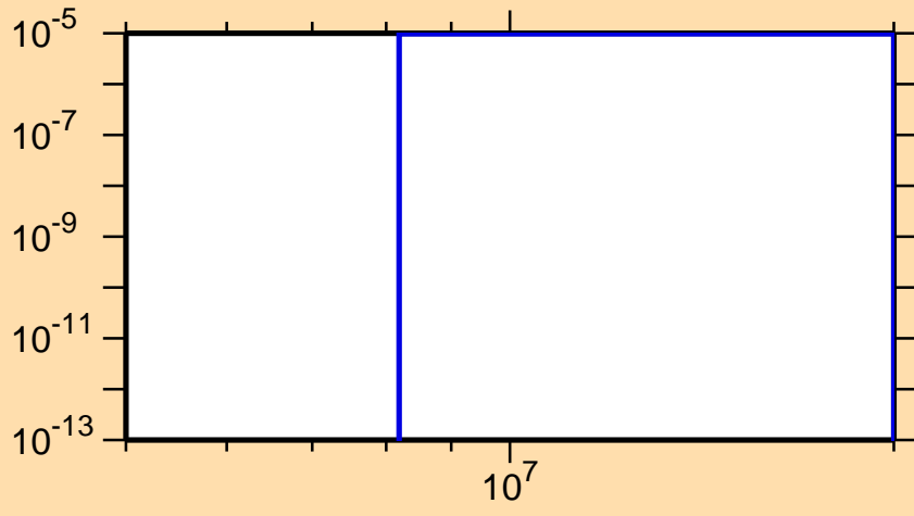
\sigma vs. E for ^{142}\text{Sm}(n,t)
