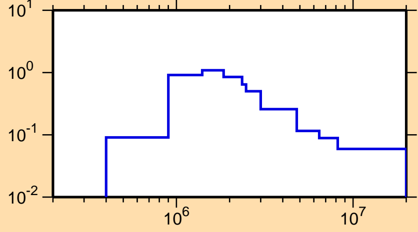
\sigma vs. E for ^{142}\text{Sm}(n,n_1)
