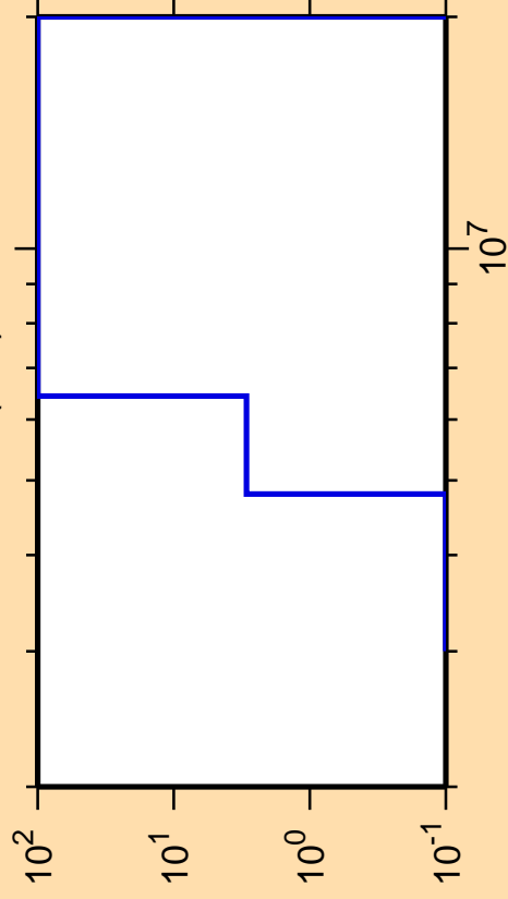
\Delta\sigma/\sigma vs. E for ^{142}\text{Sm}(n,d)
