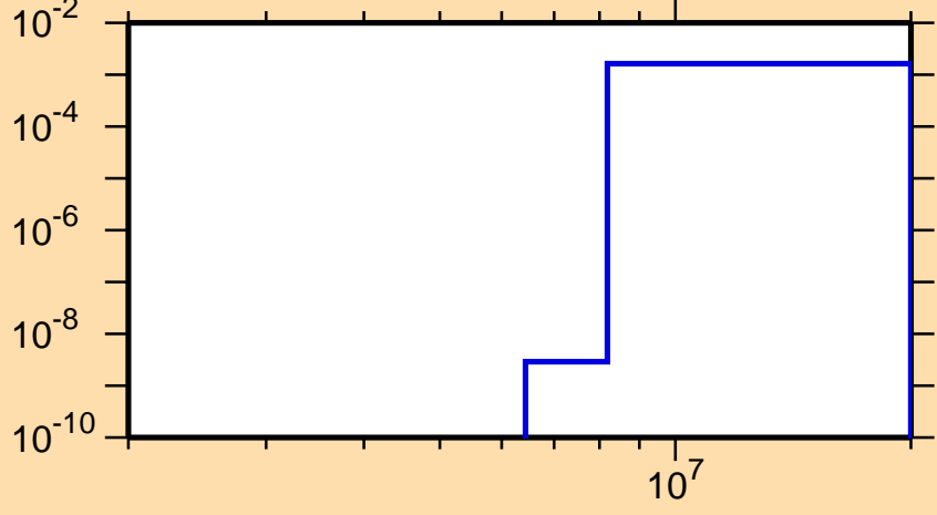
\sigma vs. E for ^{142}\text{Sm}(n,d)
