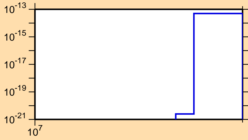
\sigma vs. E for ^{143}\text{Sm}(n,nt)
