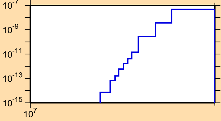
\sigma vs. E for ^{143}\text{Sm}(n,pd)
