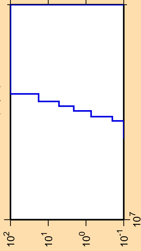
\Delta\sigma/\sigma vs. E for ^{143}\text{Sm}(n,pd)
