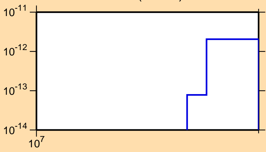
\sigma vs. E for ^{143}\text{Sm}(\text{mt117})
