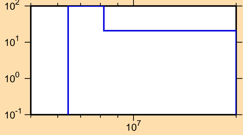
\Delta\sigma/\sigma vs. E for ^{143}\text{Sm}(n,2n)
