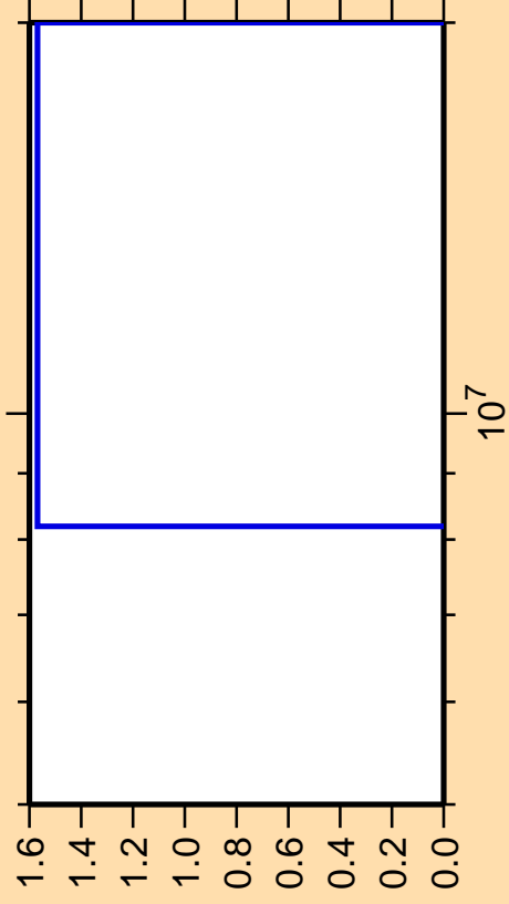
\Delta\sigma/\sigma vs. E for ^{143}\text{Sm}(\text{mt } 34)
