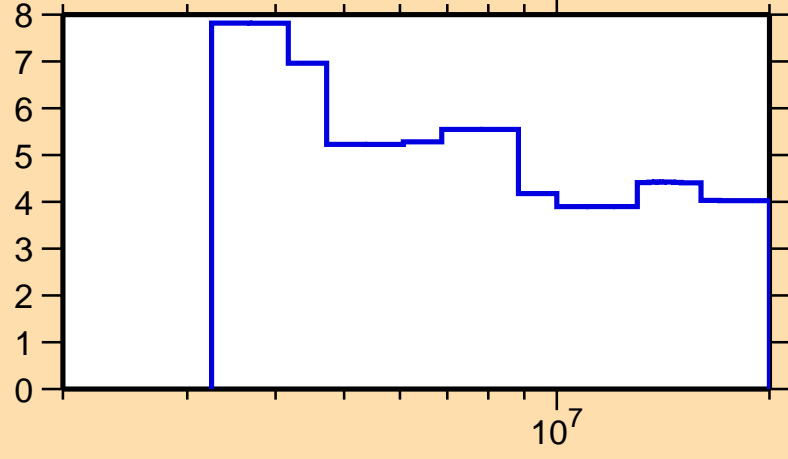
\Delta\sigma/\sigma vs. E for ^{144}\text{Sm}(n,\text{nonel.})
