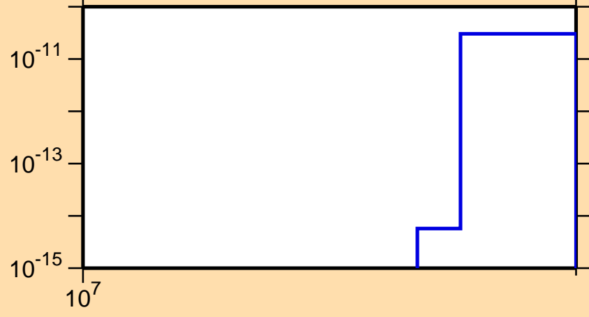
\sigma vs. E for ^{144}\text{Sm} (mt 45)
