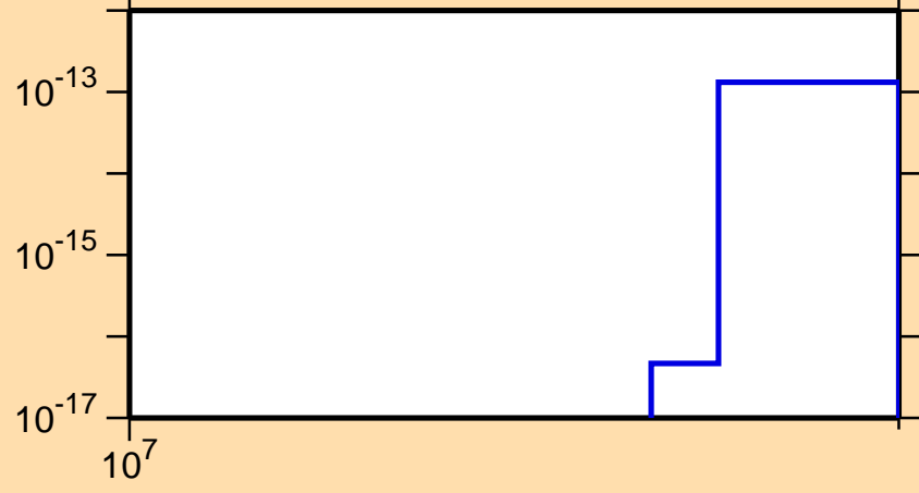
\sigma vs. E for ^{144}\text{Sm}(n,nt)
