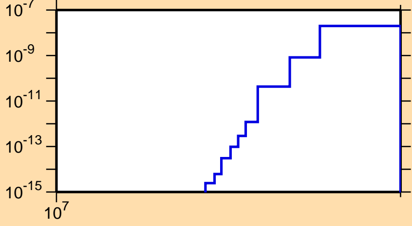
\sigma vs. E for ^{144}\text{Sm}(n,pd)
