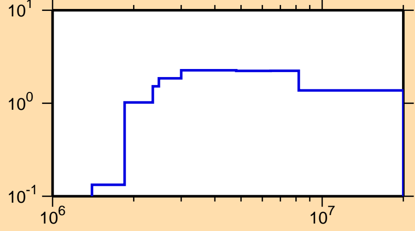
\sigma vs. E for ^{144}\text{Sm}(n,\text{inel.})
