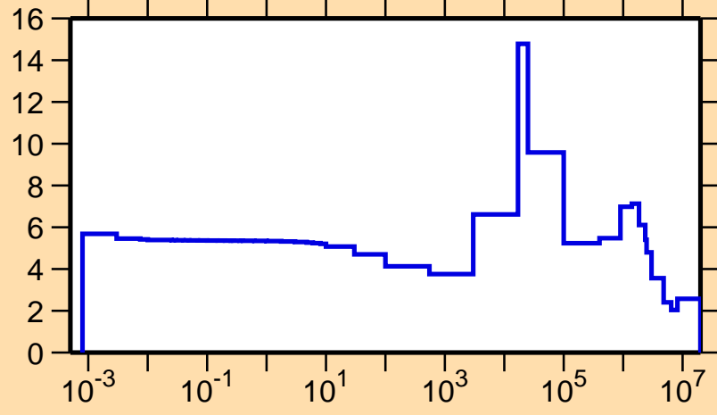
\sigma vs. E for ^{144}\text{Sm}(n,\text{el.})
