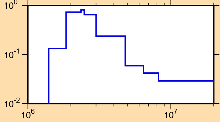
\sigma vs. E for ^{144}\text{Sm}(n,n_1)
