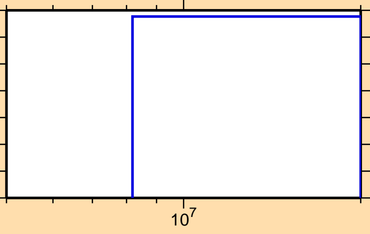
\sigma vs. E for ^{144}\text{Sm}(n,\text{He3})
