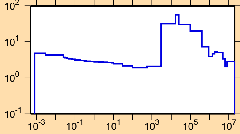
\Delta\sigma/\sigma vs. E for ^{144}\text{Sm}(n,\text{tot.})
