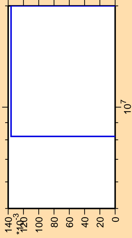
\Delta\sigma/\sigma vs. E for ^{144}\text{Sm}(\text{mt } 45)
