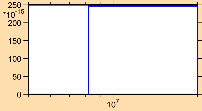
\sigma vs. E for ^{144}\text{Sm}(\text{mt } 45)
