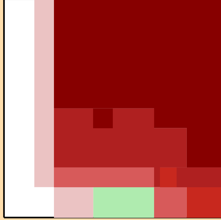
\Delta\sigma/\sigma vs. E for ^{145}\text{Sm}(n,2n)
