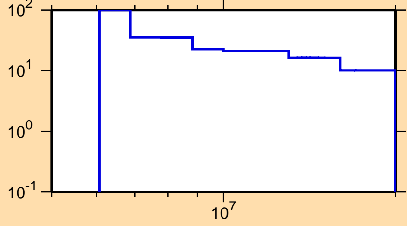
\Delta\sigma/\sigma vs. E for ^{145}\text{Sm}(n,2n)
