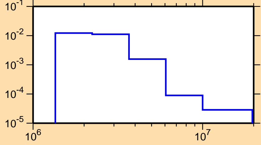
\sigma vs. E for ^{145}\text{Sm}(n,n_4)
