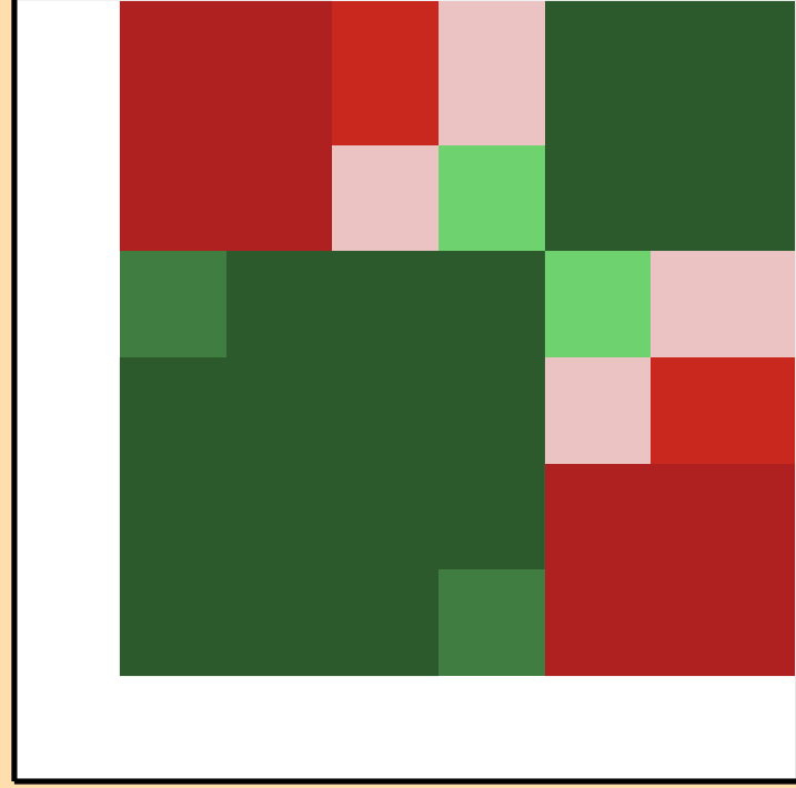
\sigma vs. E for ^{145}\text{Sm}(n,\text{inel.})
