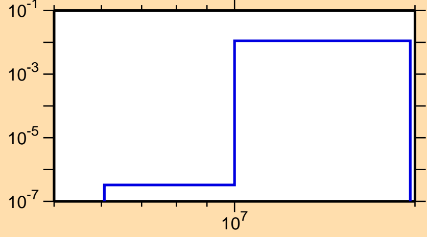
\sigma vs. E for ^{145}\text{Sm}(n,np)
