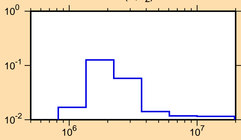
\sigma vs. E for ^{145}\text{Sm}(n,n_2)
