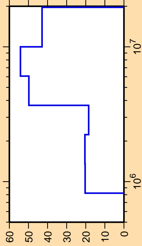
\Delta\sigma/\sigma vs. E for ^{145}\text{Sm}(n,n_2)
