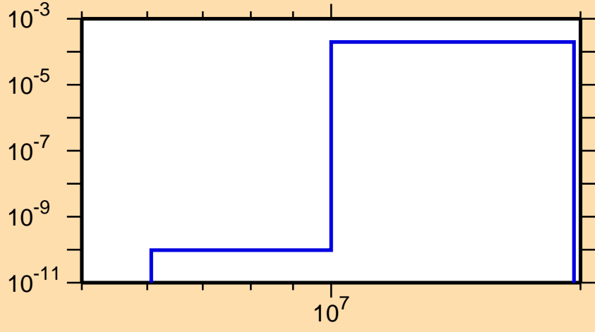
\sigma vs. E for ^{145}\text{Sm}(n,t)
