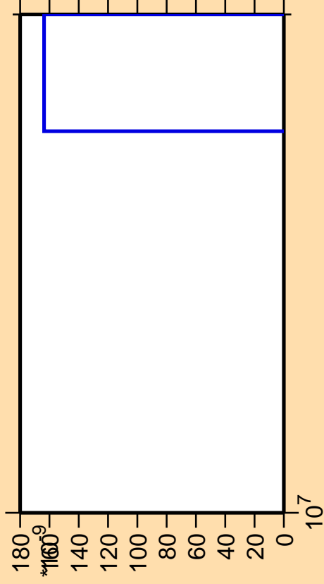
\Delta\sigma/\sigma vs. E for ^{148}\text{Sm} (mt 11)
