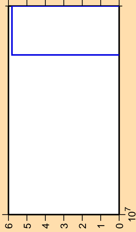
\Delta\sigma/\sigma vs. E for ^{148}\text{Sm} (mt 45)
