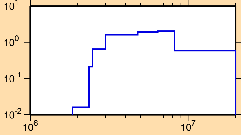
\sigma vs. E for ^{148}\text{Sm}(n,n\text{cont.})
