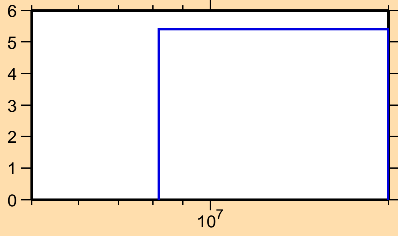
\Delta\sigma/\sigma vs. E for ^{148}\text{Sm}(n,\text{el.})
