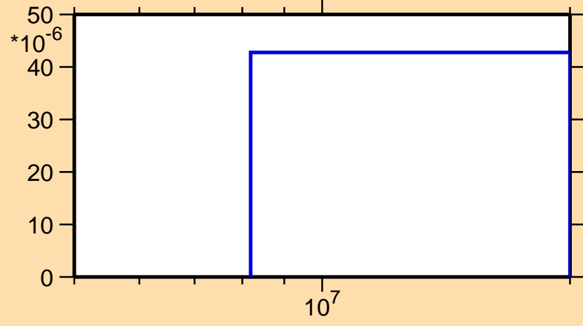
\sigma vs. E for ^{148}\text{Sm}(n,t)
