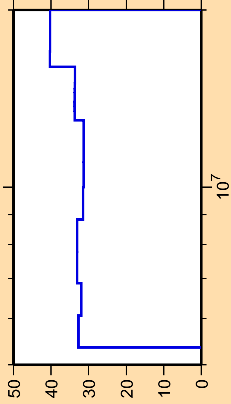
\Delta\sigma/\sigma vs. E for ^{151}\text{Sm}(n,\alpha)
