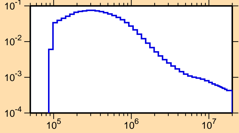
\sigma vs. E for ^{151}\text{Sm}(n,n_4)
