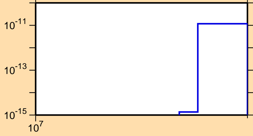
\sigma vs. E for ^{151}\text{Sm}(n,3n\alpha)
