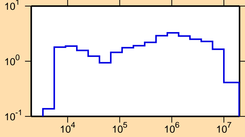
\sigma vs. E for ^{151}\text{Sm}(n,\text{inel.})
