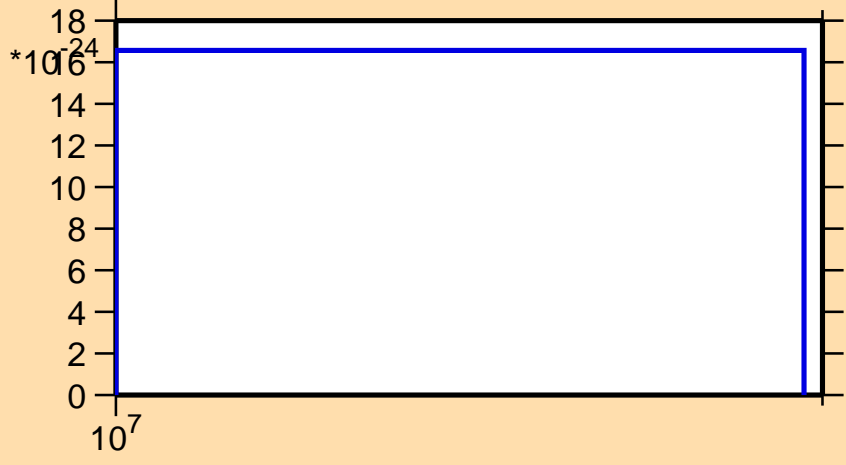
\sigma vs. E for ^{151}\text{Sm} (mt 11)
