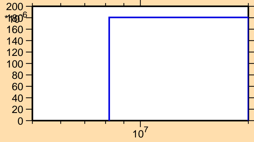
\sigma vs. E for ^{151}\text{Sm}(n,t)
