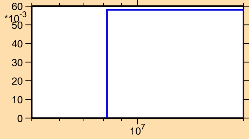
\sigma vs. E for ^{151}\text{Sm}(n,3n)
