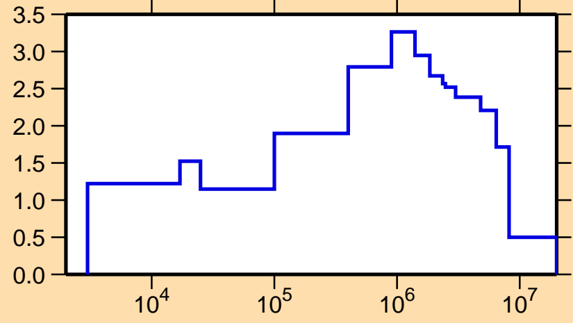
\sigma vs. E for ^{151}\text{Sm}(n,\text{inel.})
