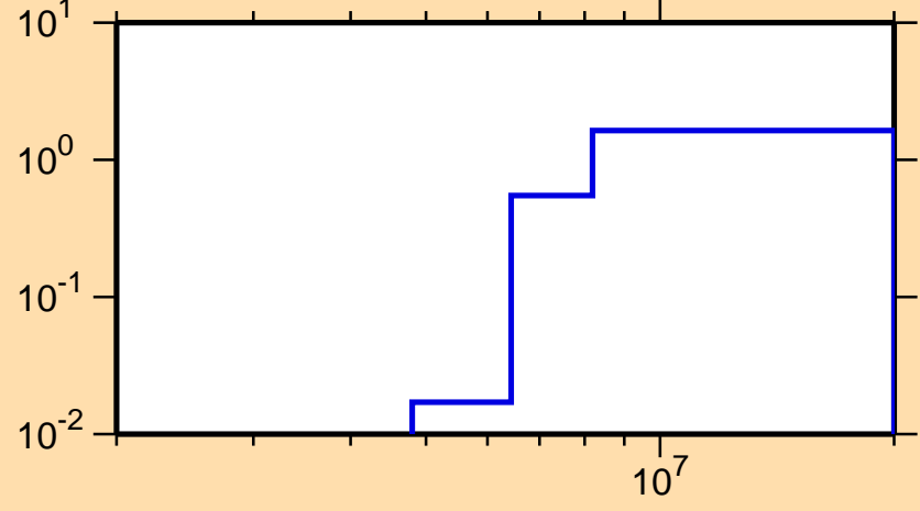
\sigma vs. E for ^{151}\text{Sm}(n,2n)
