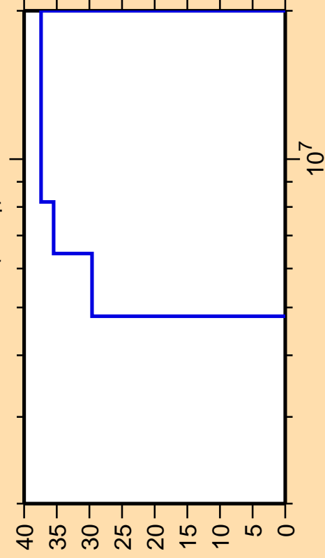
\Delta\sigma/\sigma vs. E for ^{151}\text{Sm}(n,n_1)
