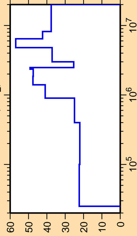
\Delta\sigma/\sigma vs. E for ^{151}\text{Sm}(n,n_2)
