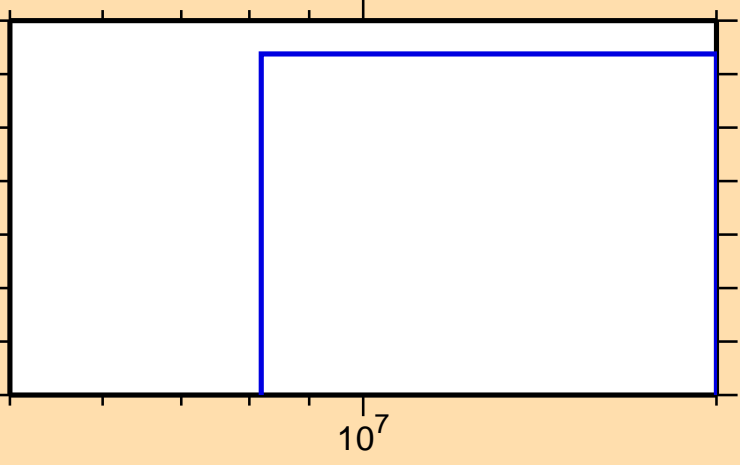
\sigma vs. E for ^{151}\text{Sm}(n,d)
