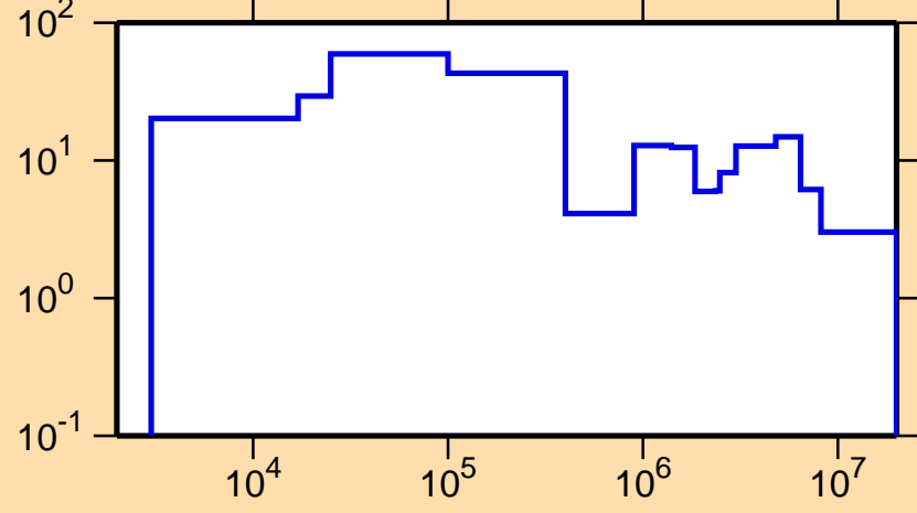
\Delta\sigma/\sigma vs. E for ^{151}\text{Sm}(n,\text{tot.})
