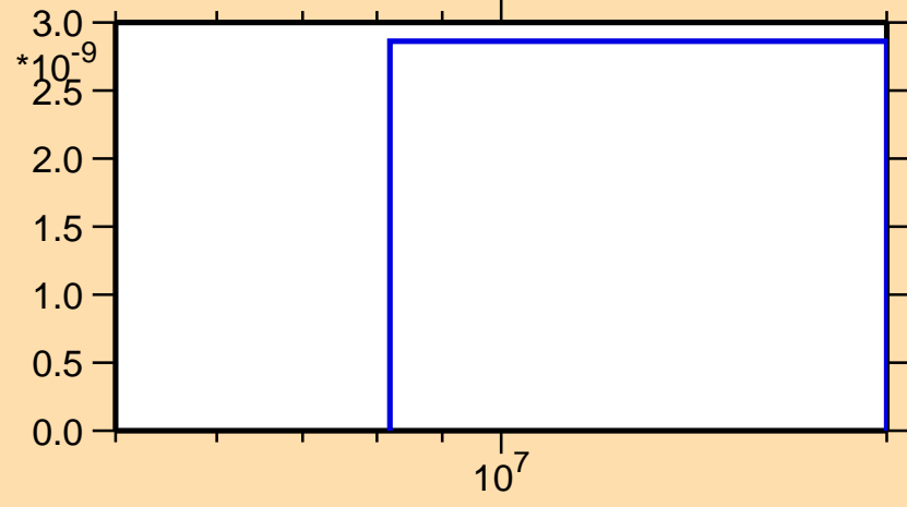
\sigma vs. E for ^{151}\text{Sm}(n,nt)
