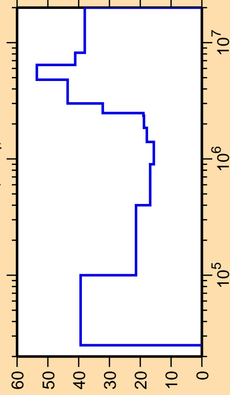
\Delta\sigma/\sigma vs. E for ^{151}\text{Sm}(n,n_4)
