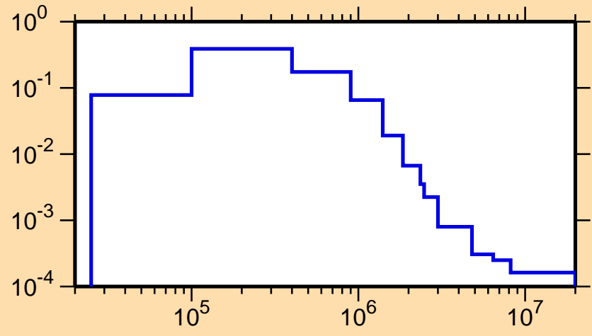
\sigma vs. E for ^{151}\text{Sm}(n,n_2)
