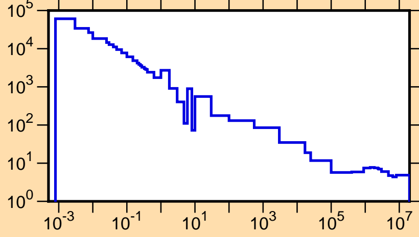
\sigma vs. E for ^{151}\text{Sm}(n,\text{tot.})
