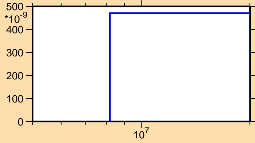
\sigma vs. E for ^{151}\text{Sm}(n,2n\alpha)
